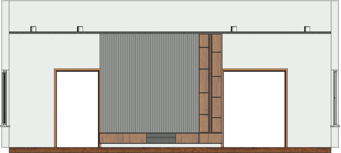
TV & Entertainment Wall — Joinery Elevation
