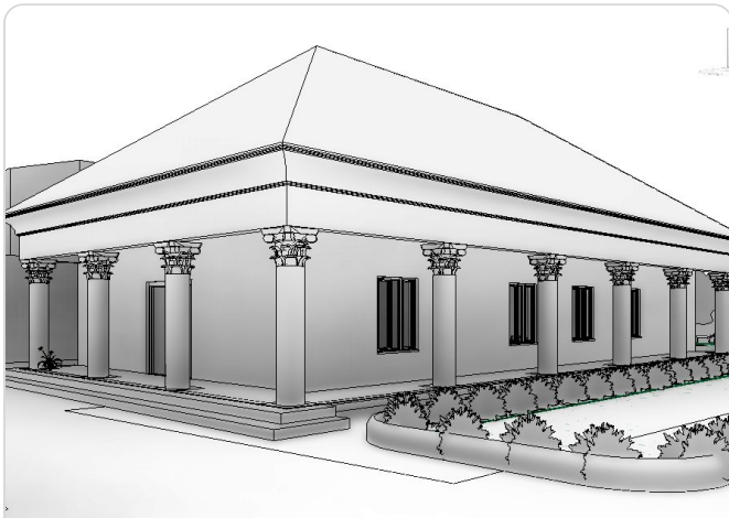
Event Hall — Hidden-Line Axonometric
