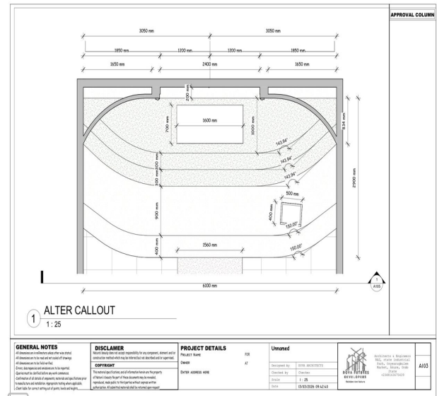
ADO CENTRE | DRAWING SET - SHEET 2
