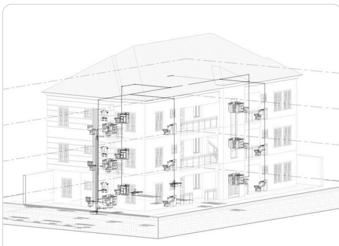
Plumbing Services Schematic
