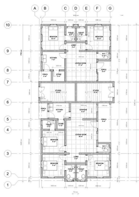
Typical Floor Plan — Dimensioned Working Drawing
