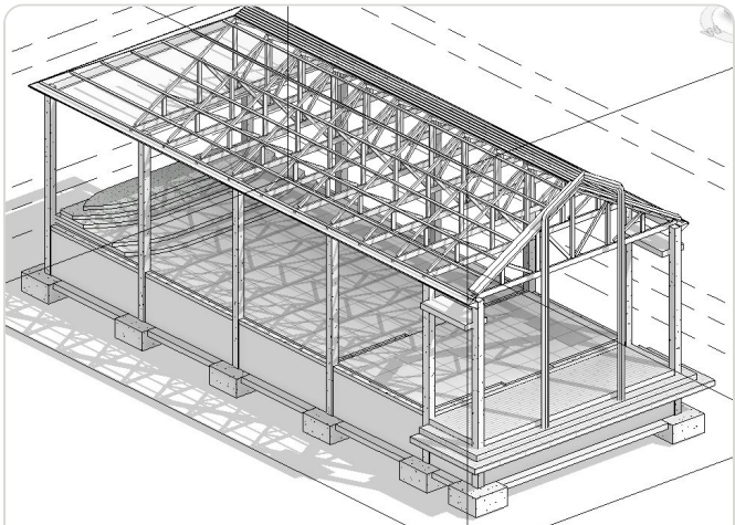
Structural Frame — Hidden-Line Axonometric
