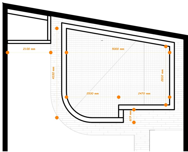
Pool Plan — Dimensioned Setting-Out Drawing
