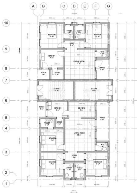
Typical Floor Plan — Dimensioned Working Drawing
