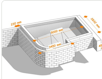
Pool Structure Isometric ISOMETRIC
