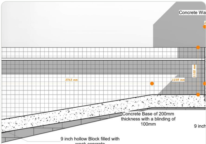
Wall & Drainage Section Detail
