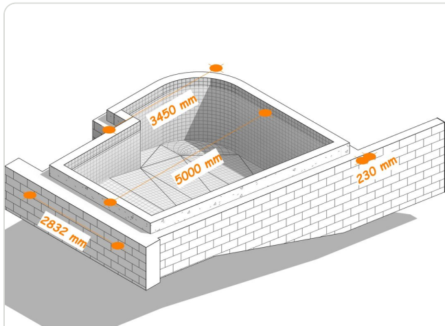
Structural Isometric — Dimensioned
