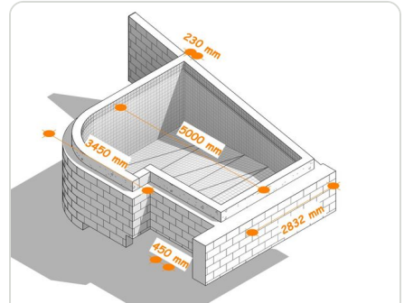
Pool Isometric — Cutaway ISOMETRIC
