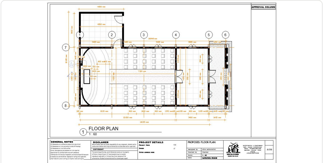
Proposed Floor Plan — Dimensioned Documentation Sheet, 1:60
