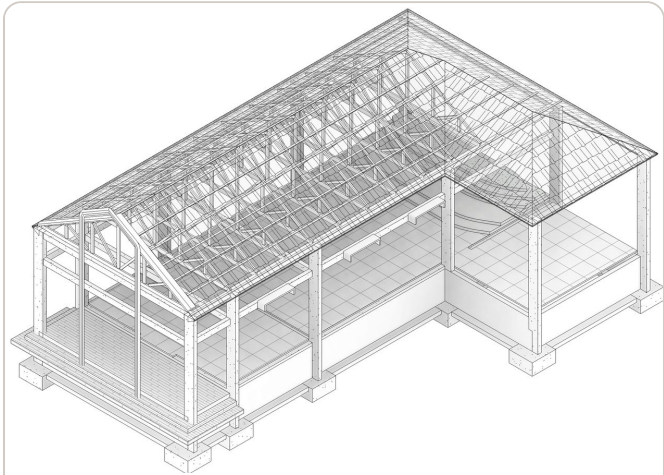
Structural BIM Model
