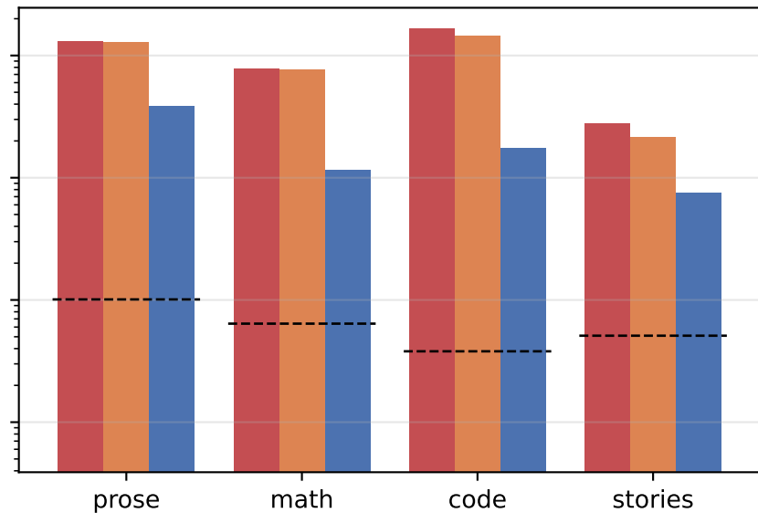
4 × KV compression ( G = 8 )
