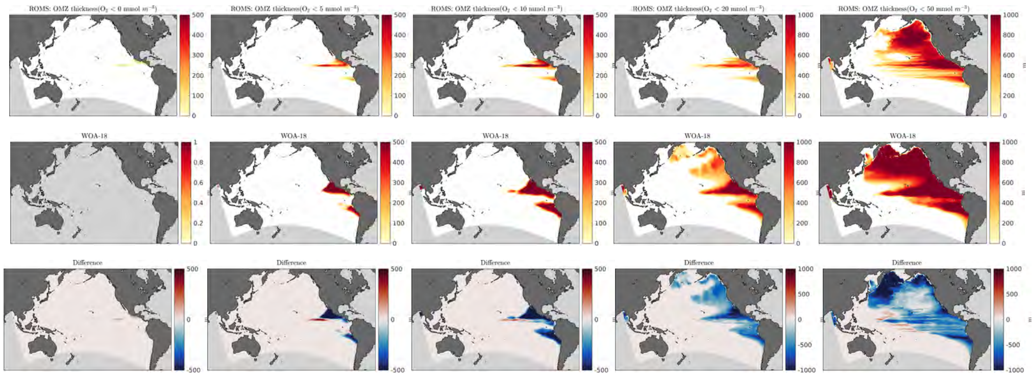
Figure 47: OMZ Thickness
