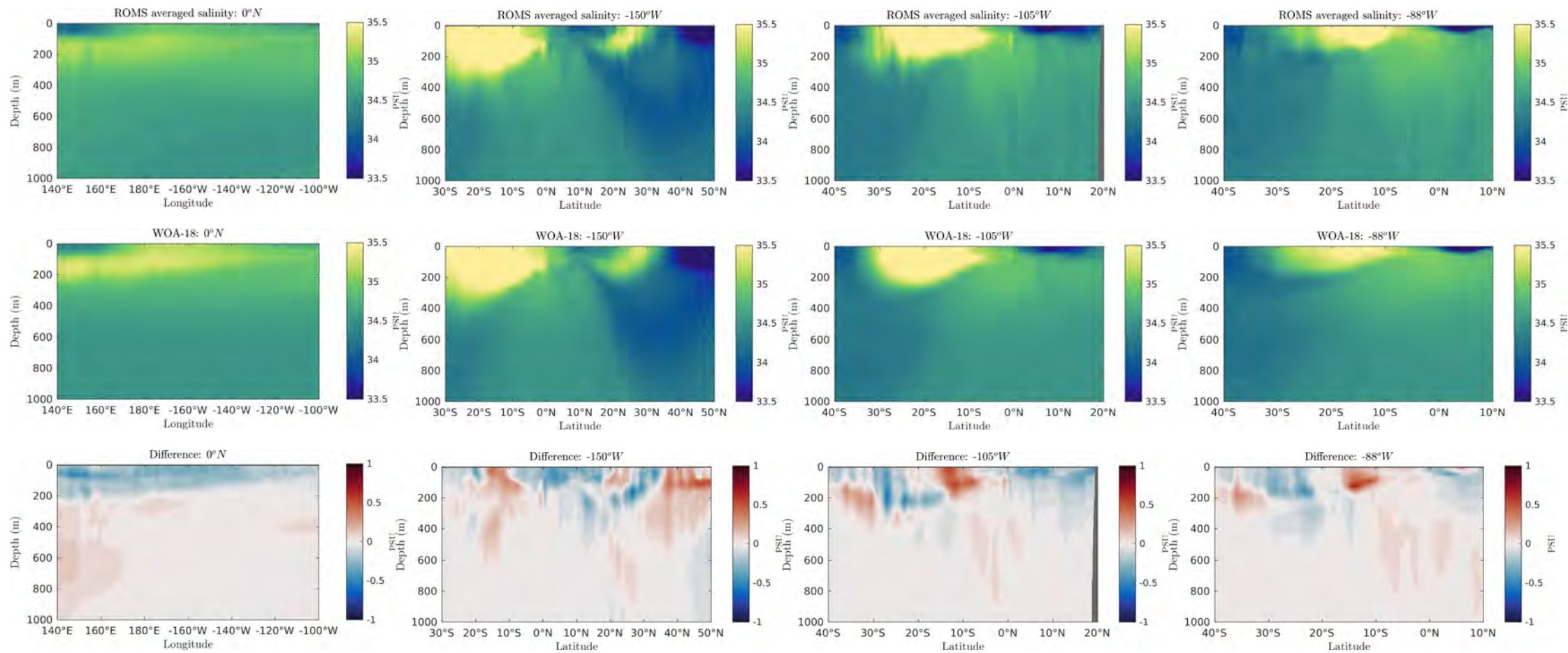
Figure 23: Salinity transects
