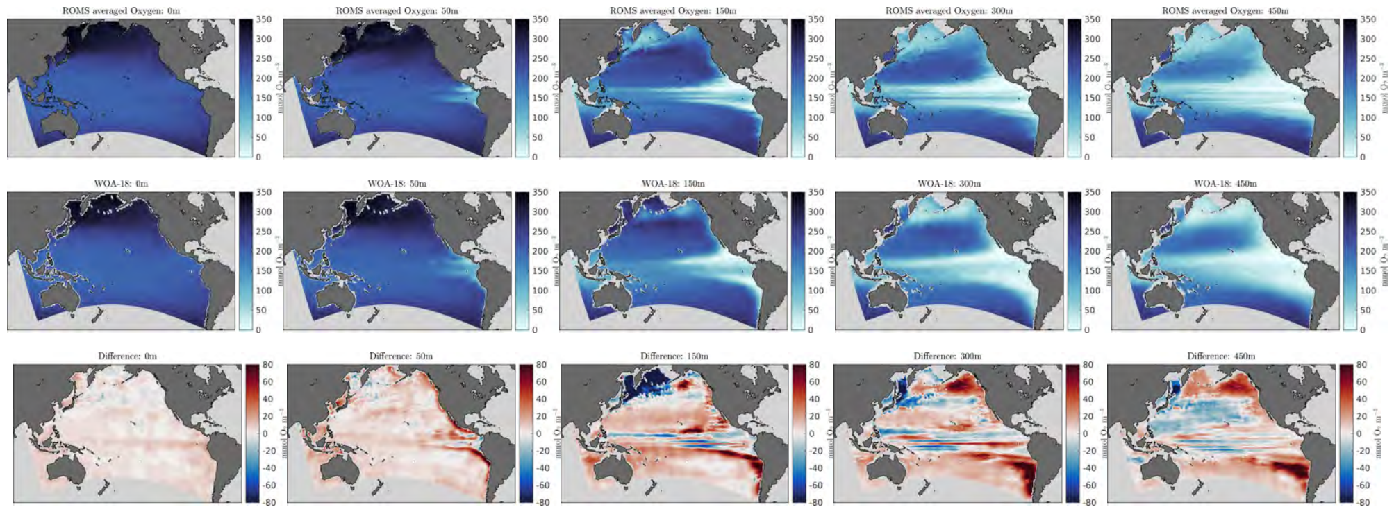
Figure 5: Oxygen Z-Slices
