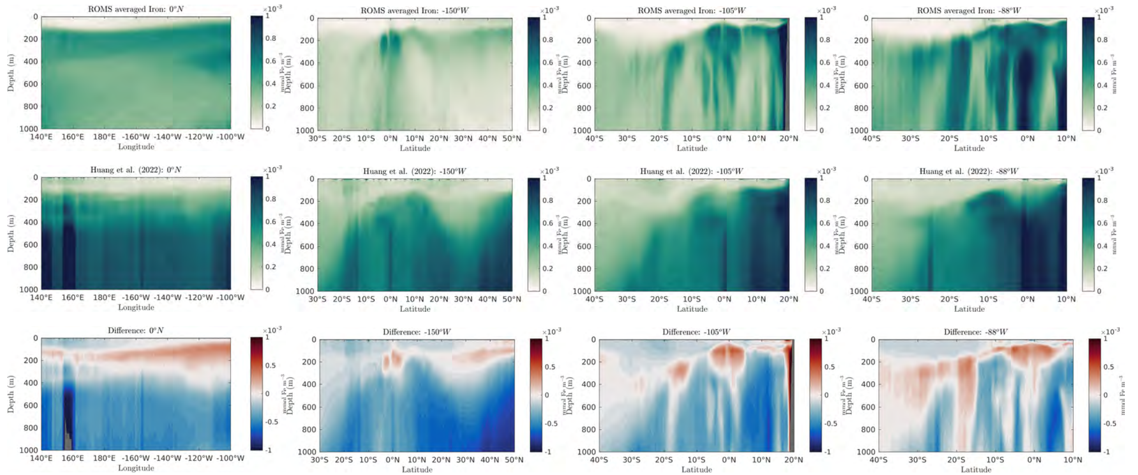
Figure 35: Iron transects
