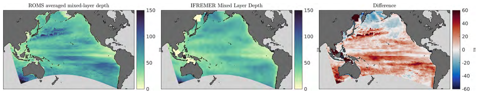
Figure 41: Mixed Layer Depth
