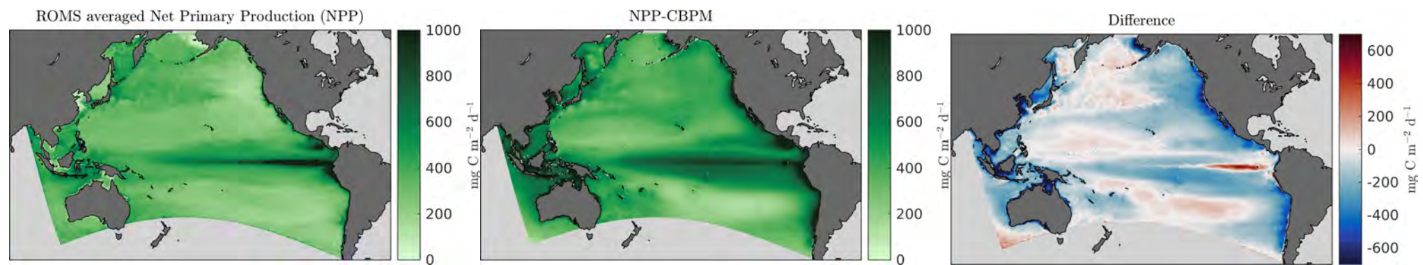
Figure 44: Net Primary Production
