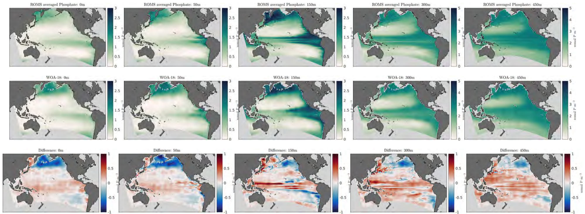
Figure 9: Phosphate Z-Slices
