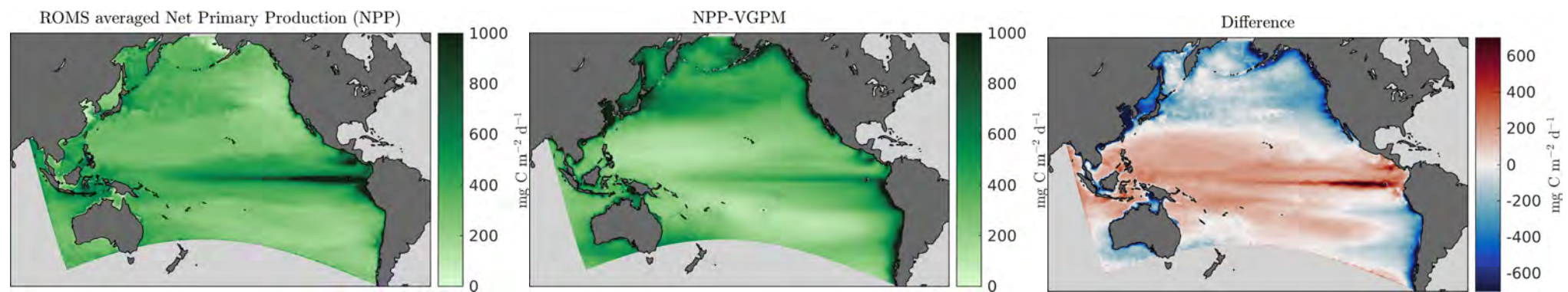
Figure 43: Net Primary Production
