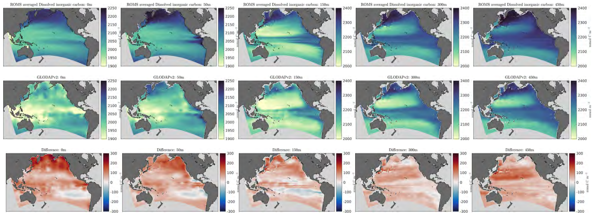
Figure 18: DIC Z-Slices
