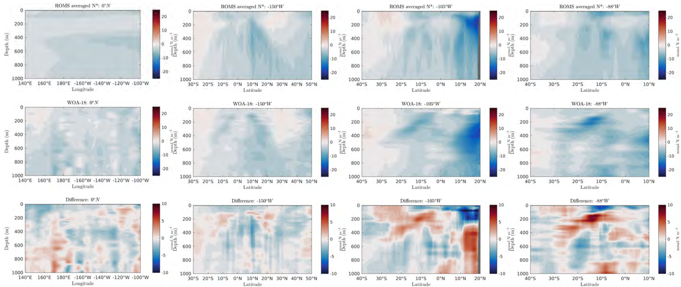
Figure 34: N^* transects
