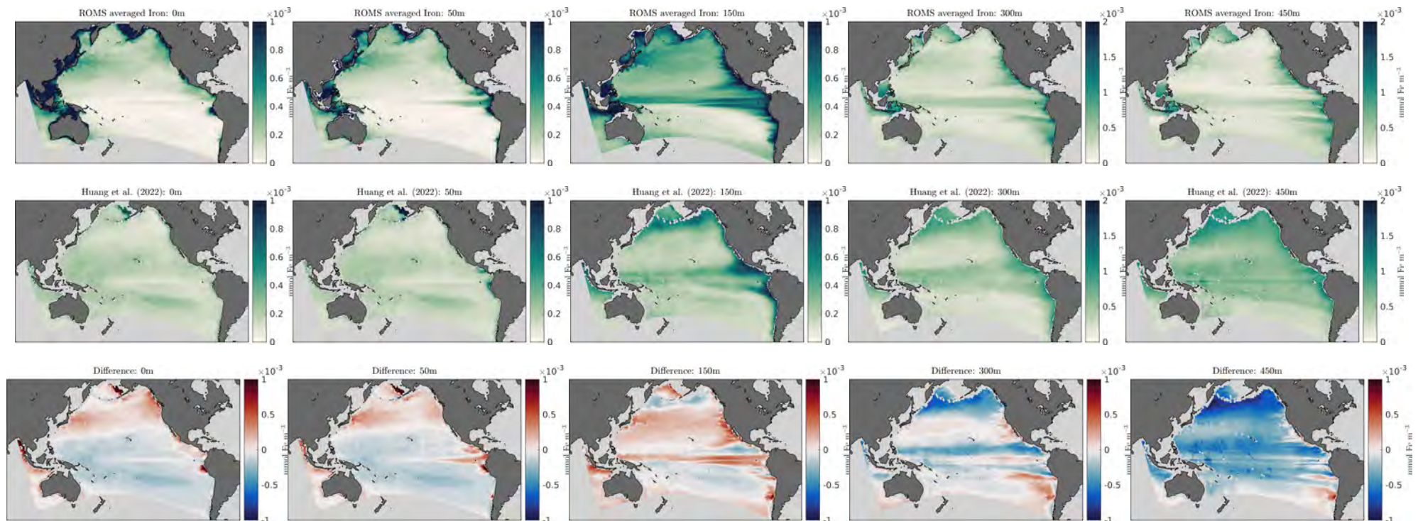
Figure 15: Iron Z-Slices
