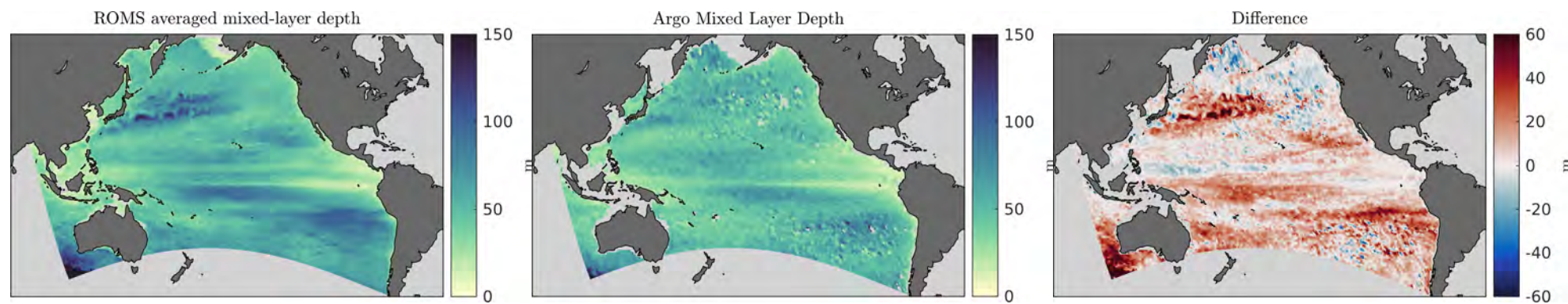
Figure 40: Mixed Layer Depth
