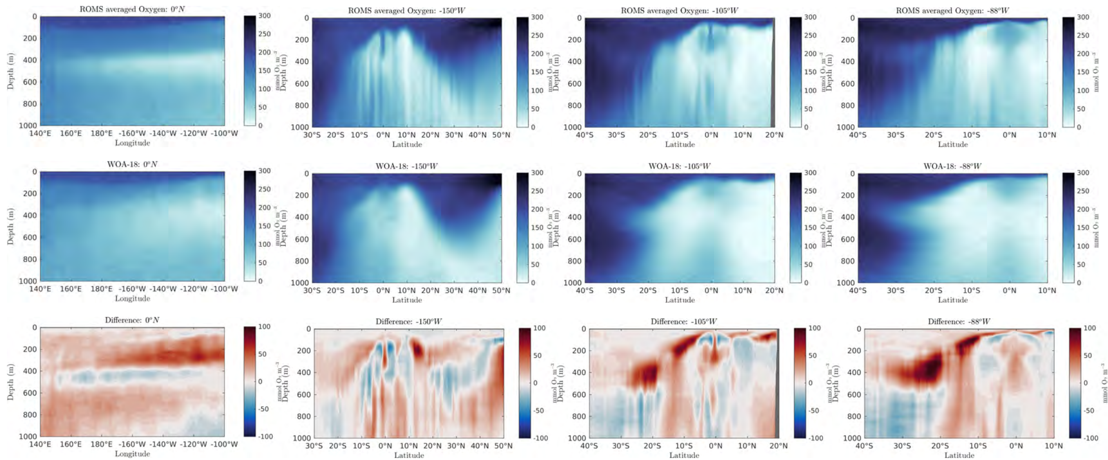
Figure 25: Oxygen transects
