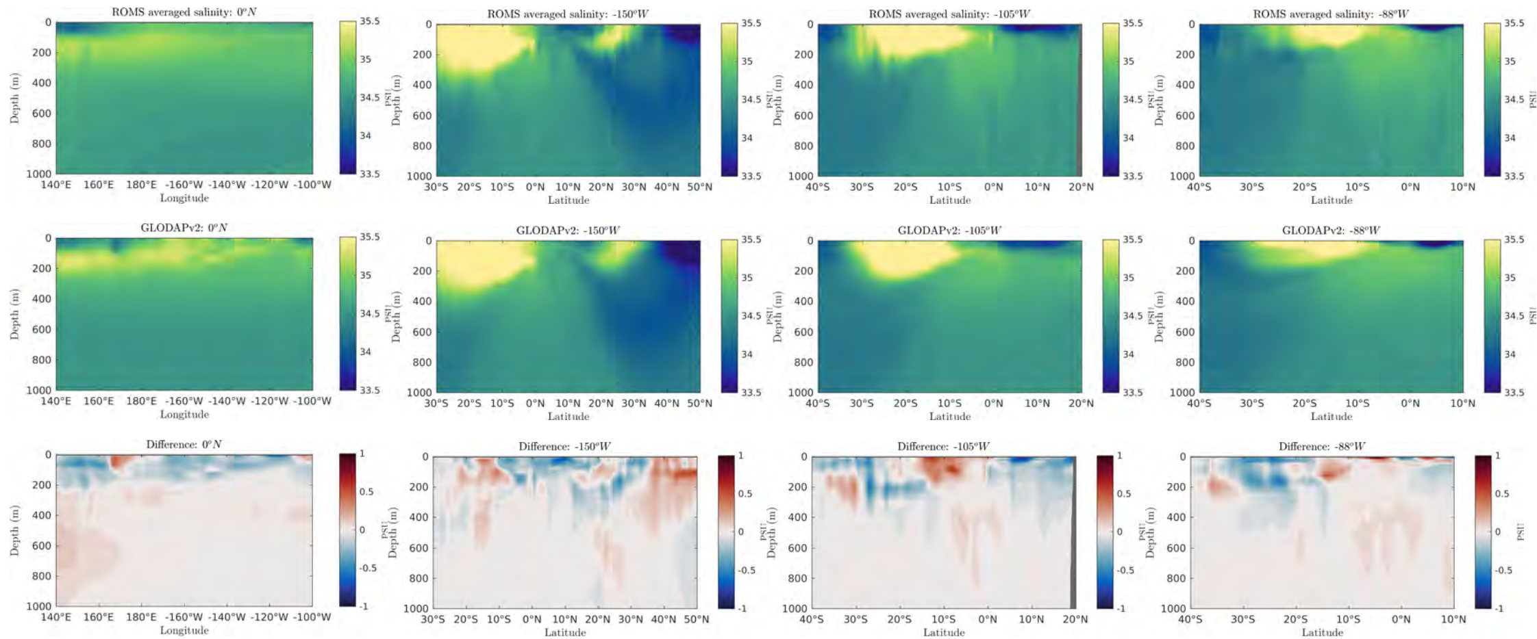
Figure 24: Salinity transects
