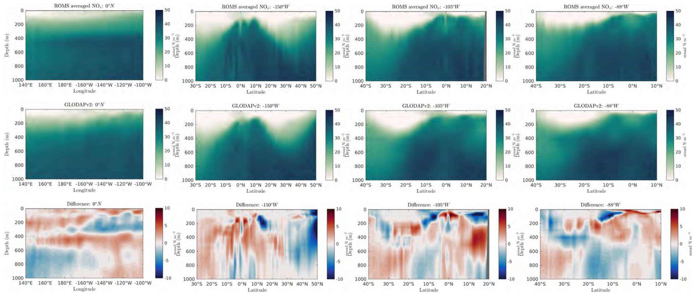
Figure 28: Nitrate+Nitrite transects
