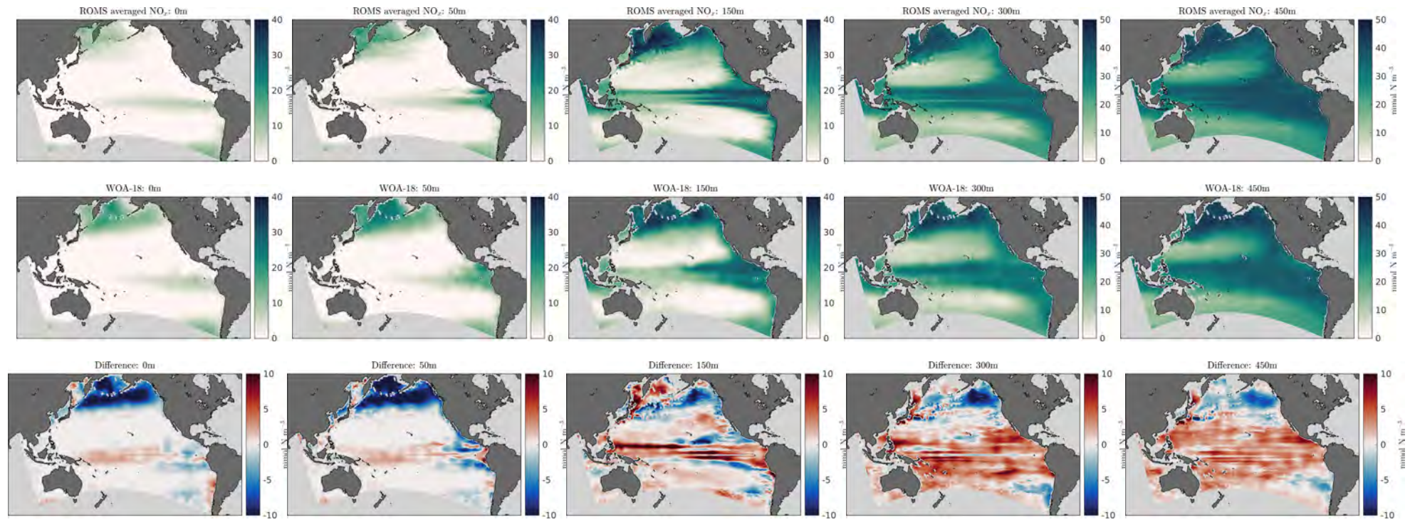
Figure 7: Nitrate+Nitrite Z-Slices
