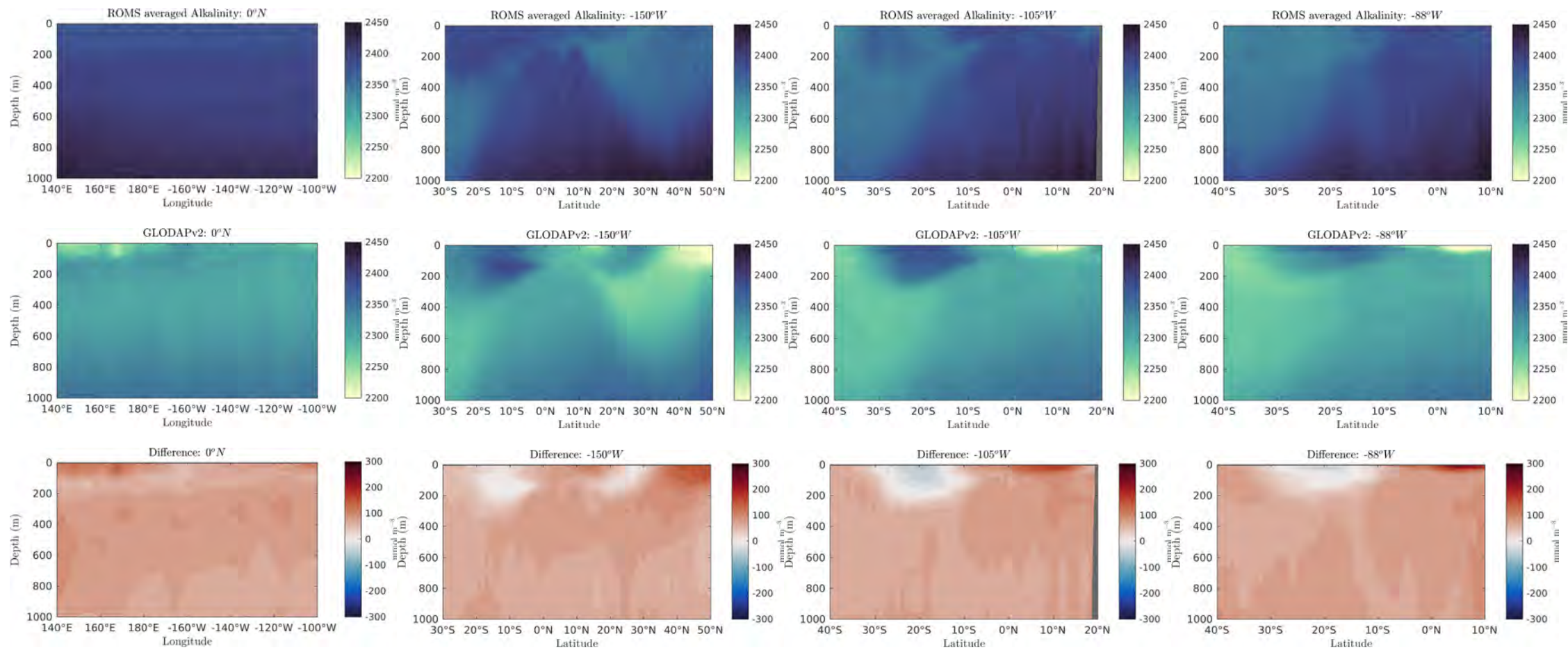
Figure 39: Alkalinity transects
