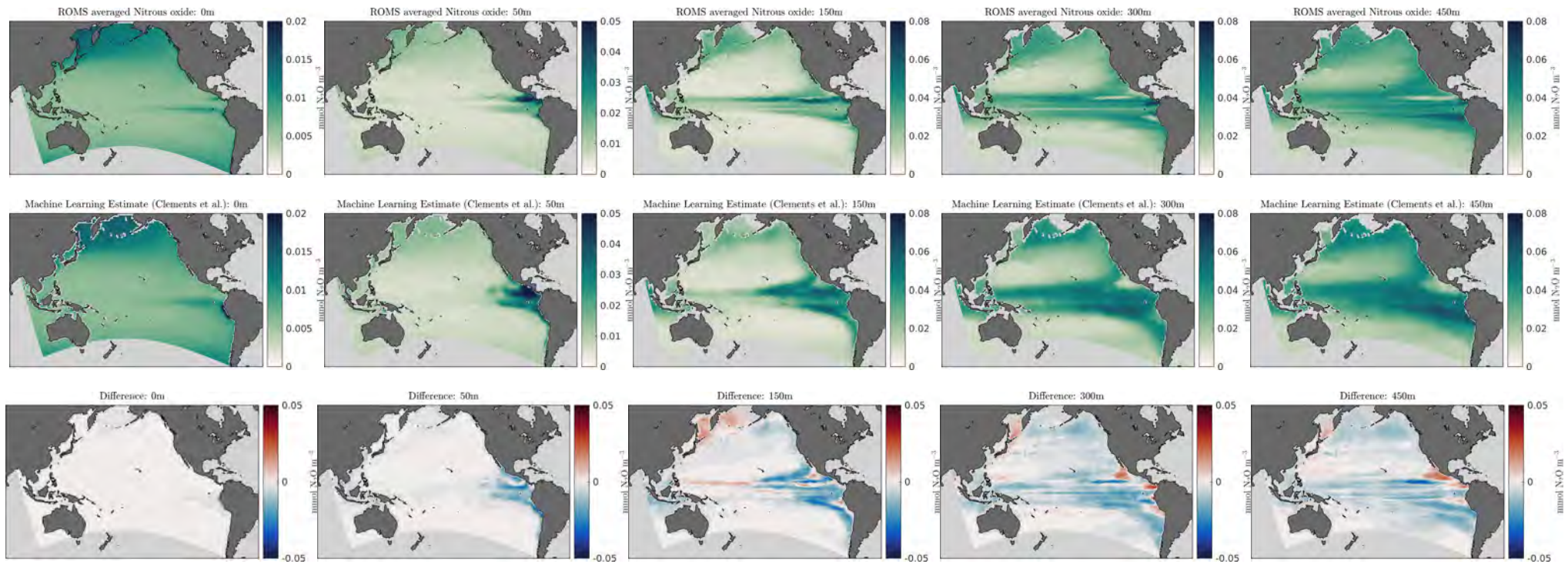
Figure 12: Nitrous Oxide Z-Slices
