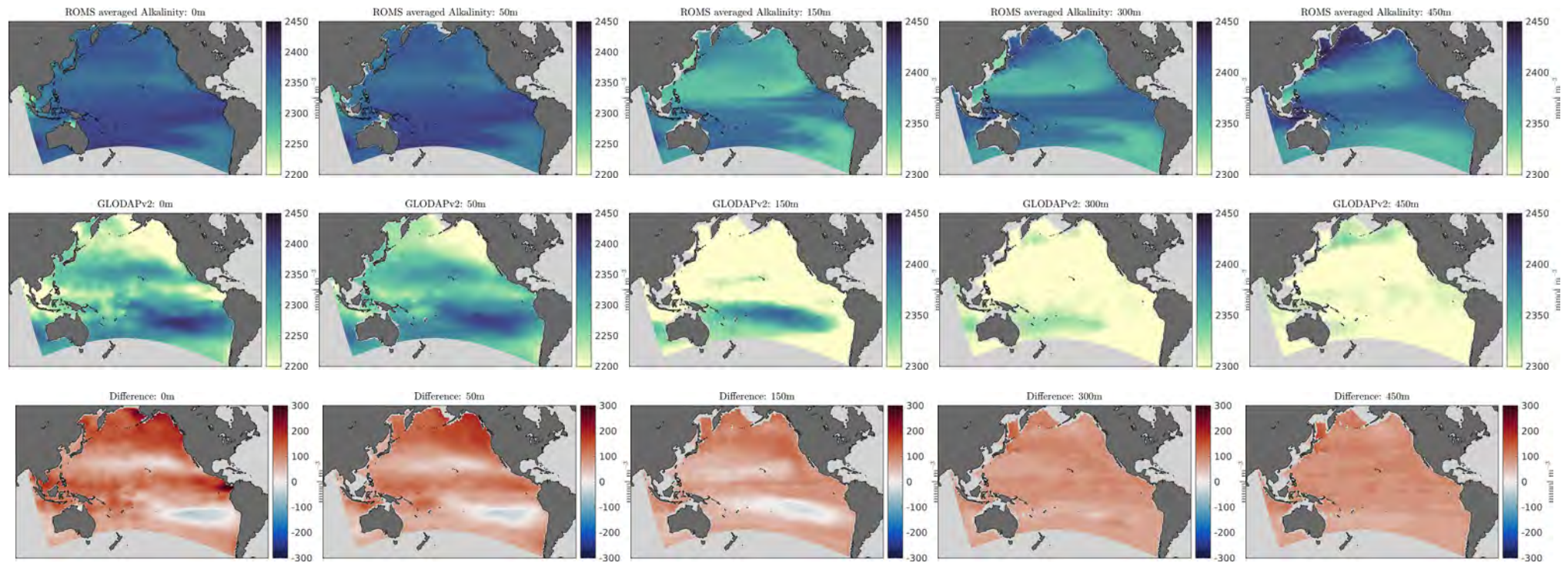
Figure 19: Alkalinity Z-Slices
