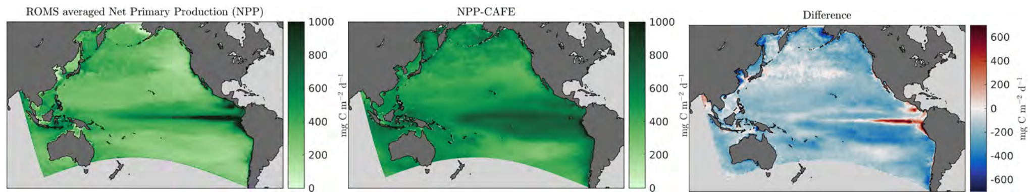
Figure 45: Net Primary Production
