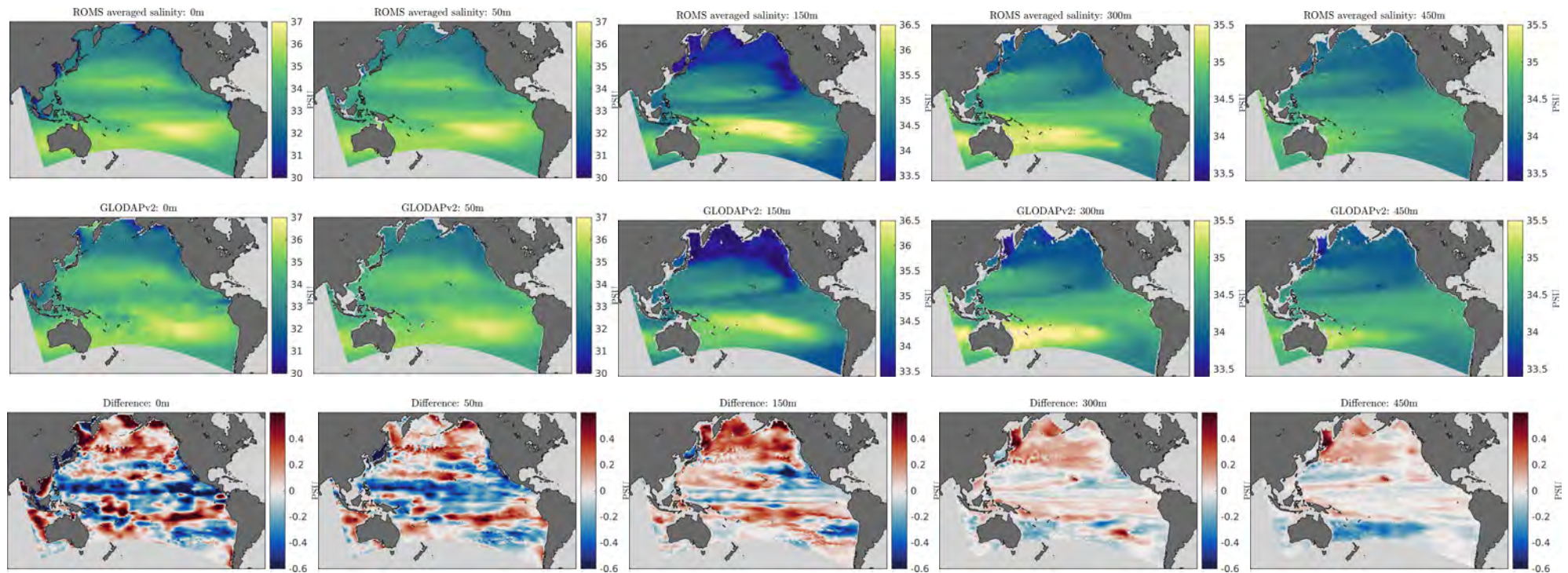
Figure 4: Salinity Z-Slices
