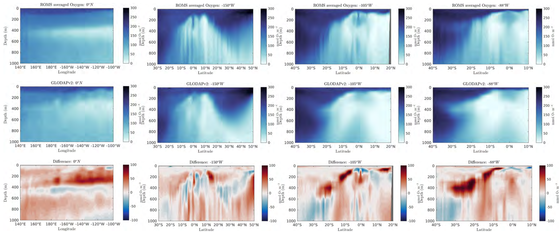
Figure 26: Oxygen transects
