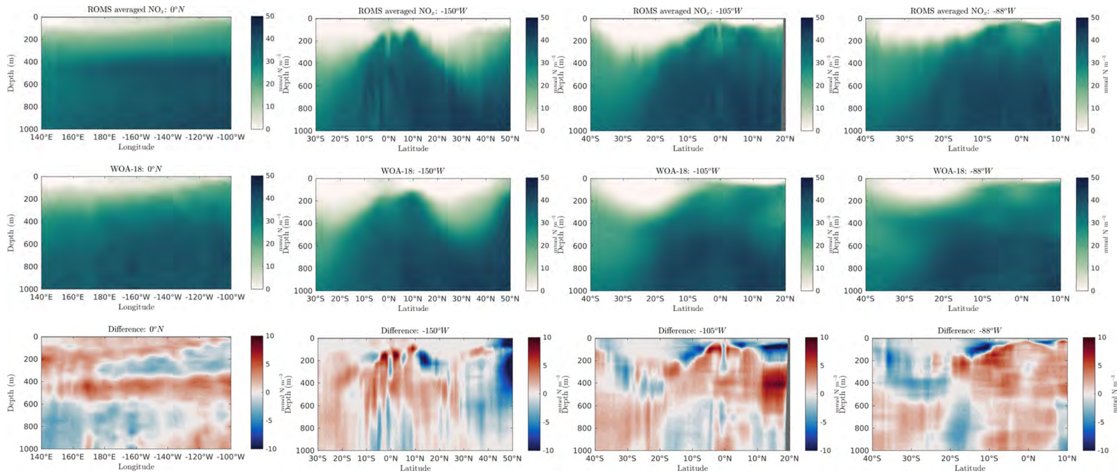
Figure 27: Nitrate+Nitrite transects
