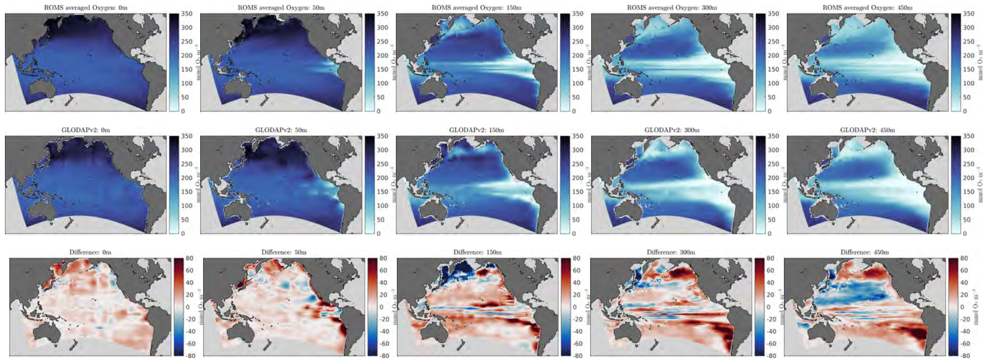
Figure 6: Oxygen Z-Slices
