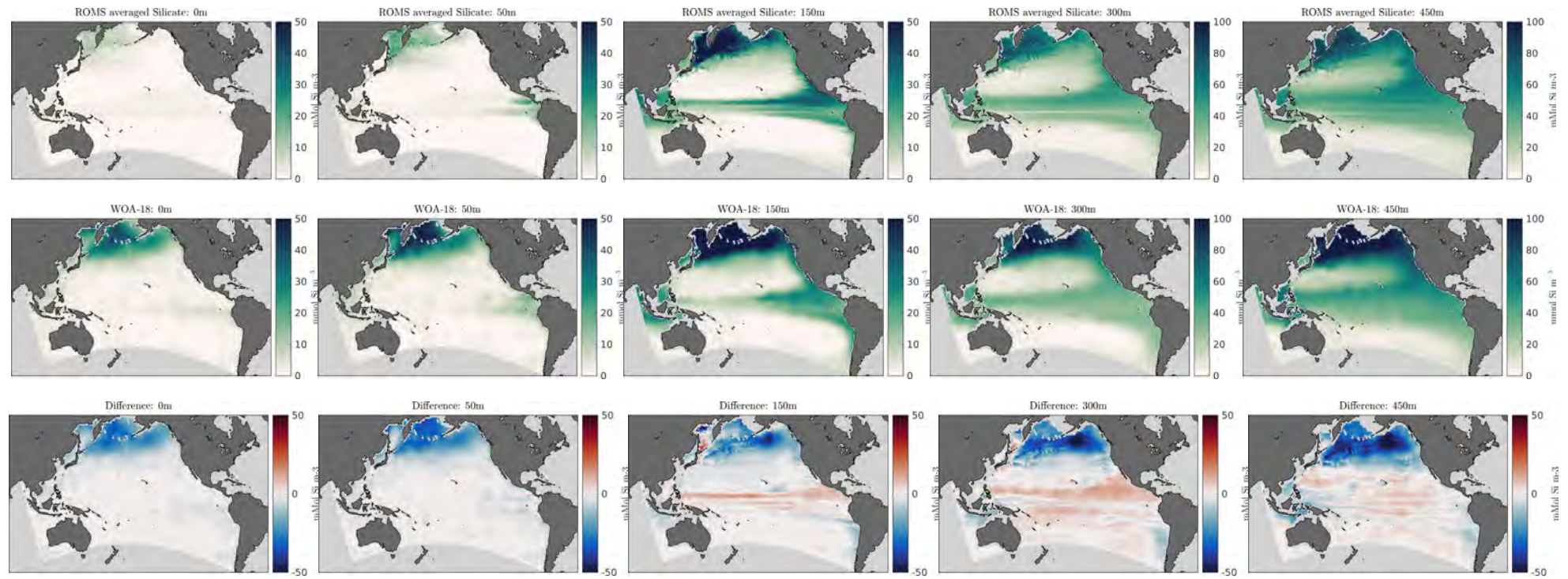
Figure 16: Silicate Z-Slices
