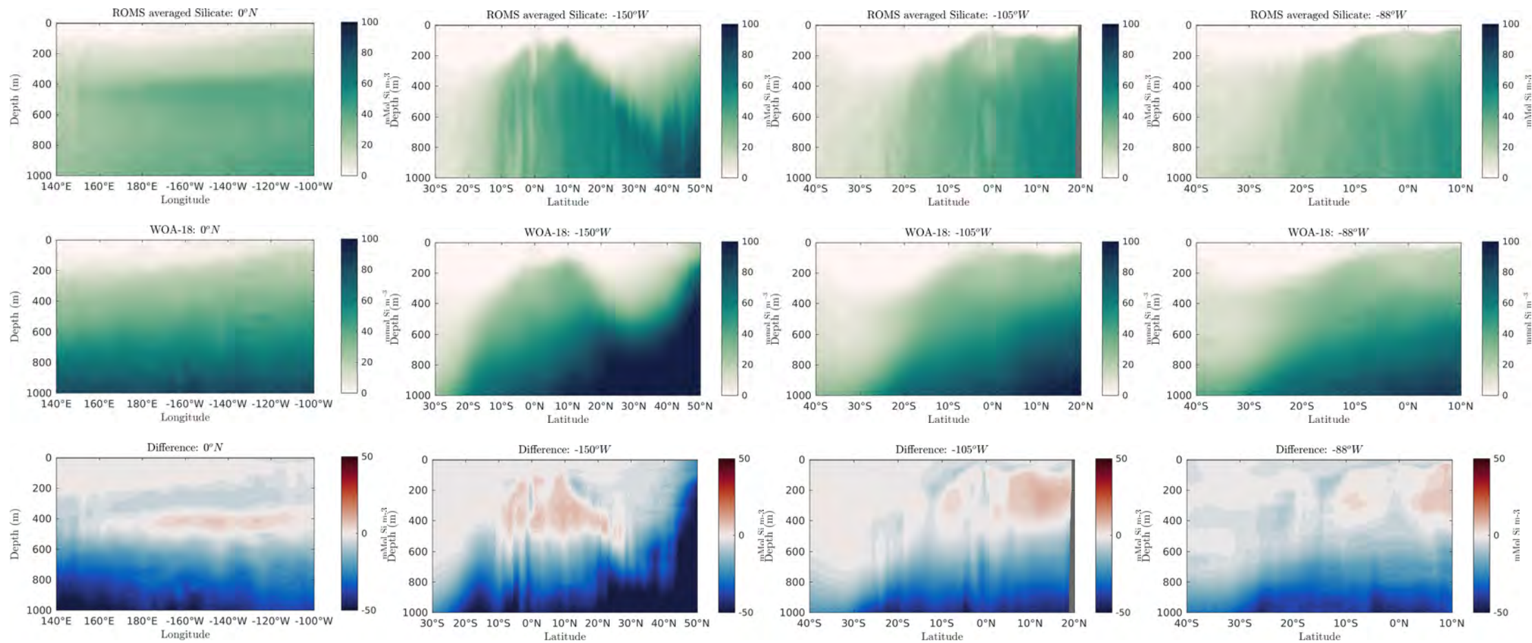
Figure 36: Silicate transects
