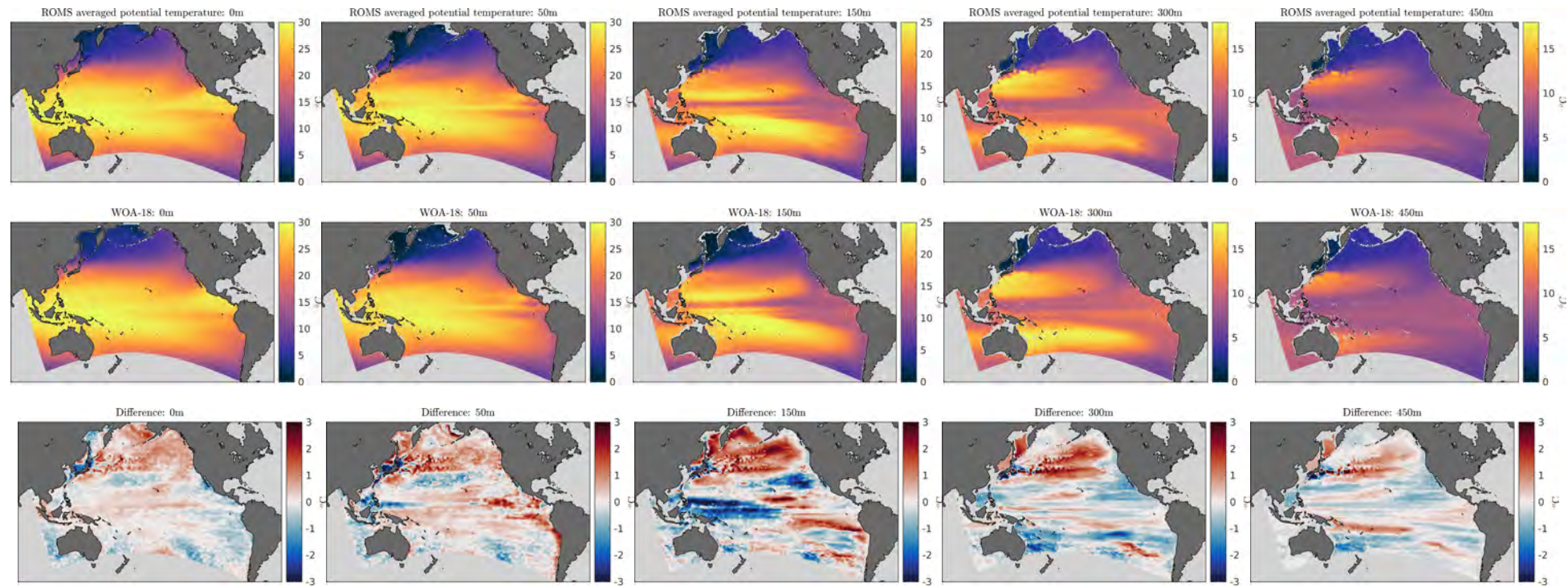
Figure 1: Temperature Z-Slices
