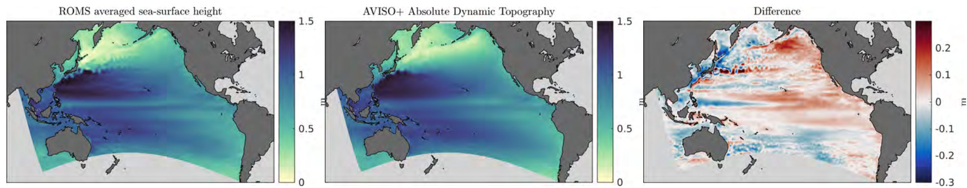
Figure 42: Sea-surface Height
