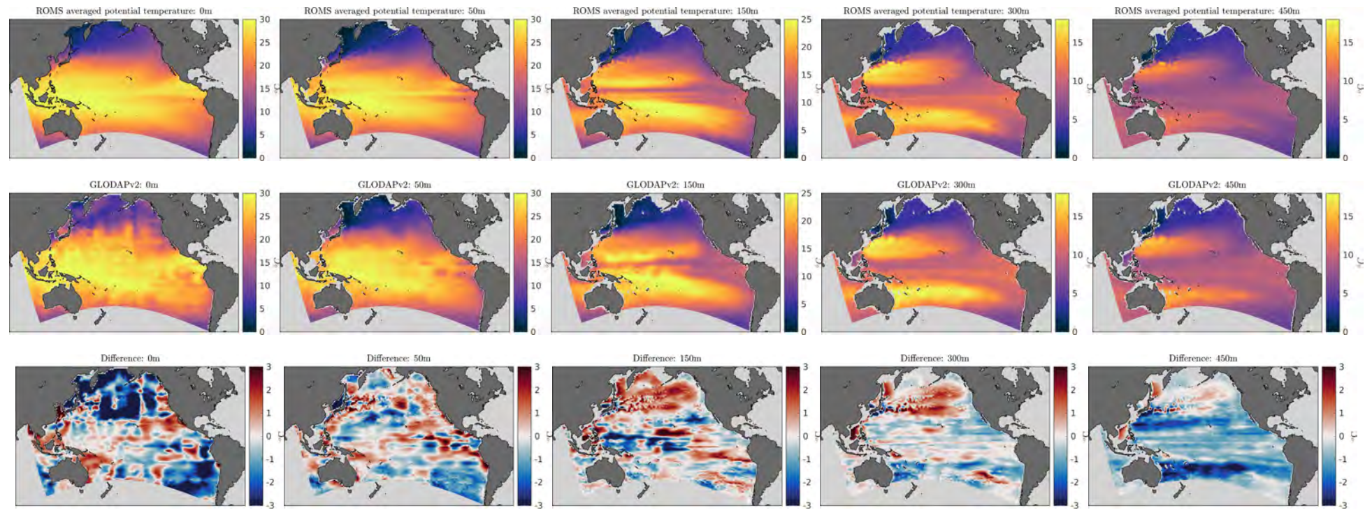
Figure 2: Temperature Z-Slices
