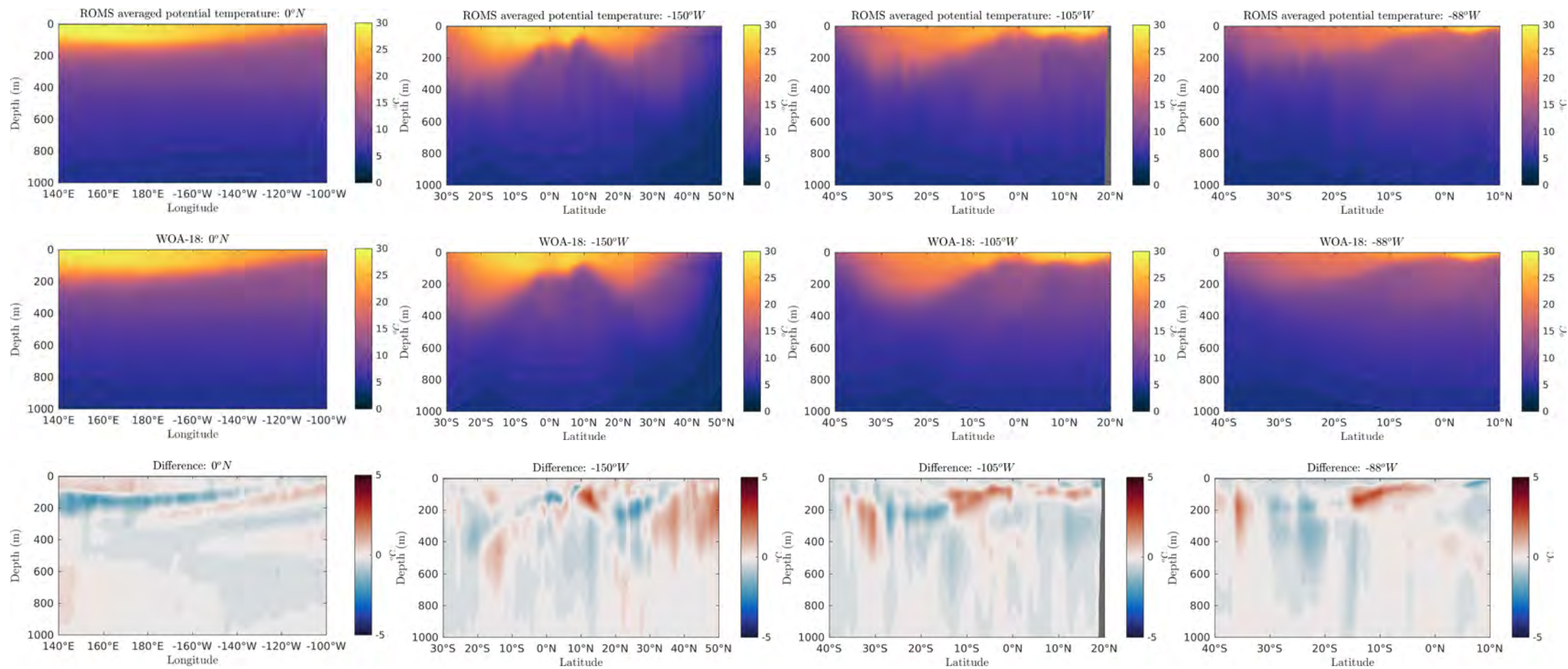
Figure 21: Temperature transects
