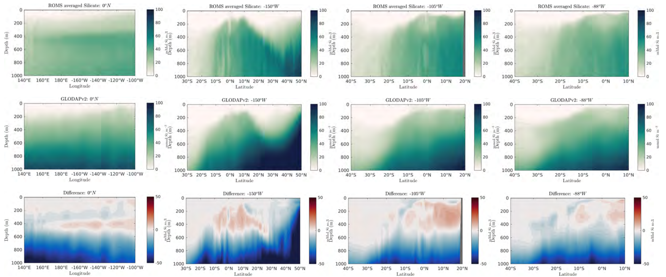
Figure 37: Silicate transects
