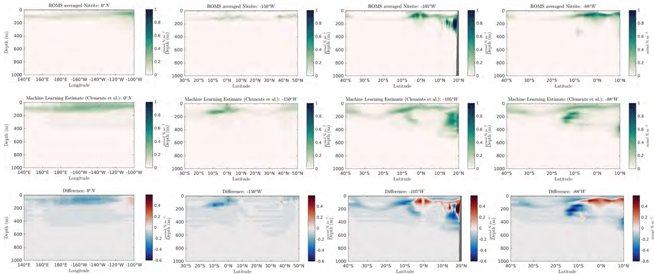
Figure 31: Nitrite transects
