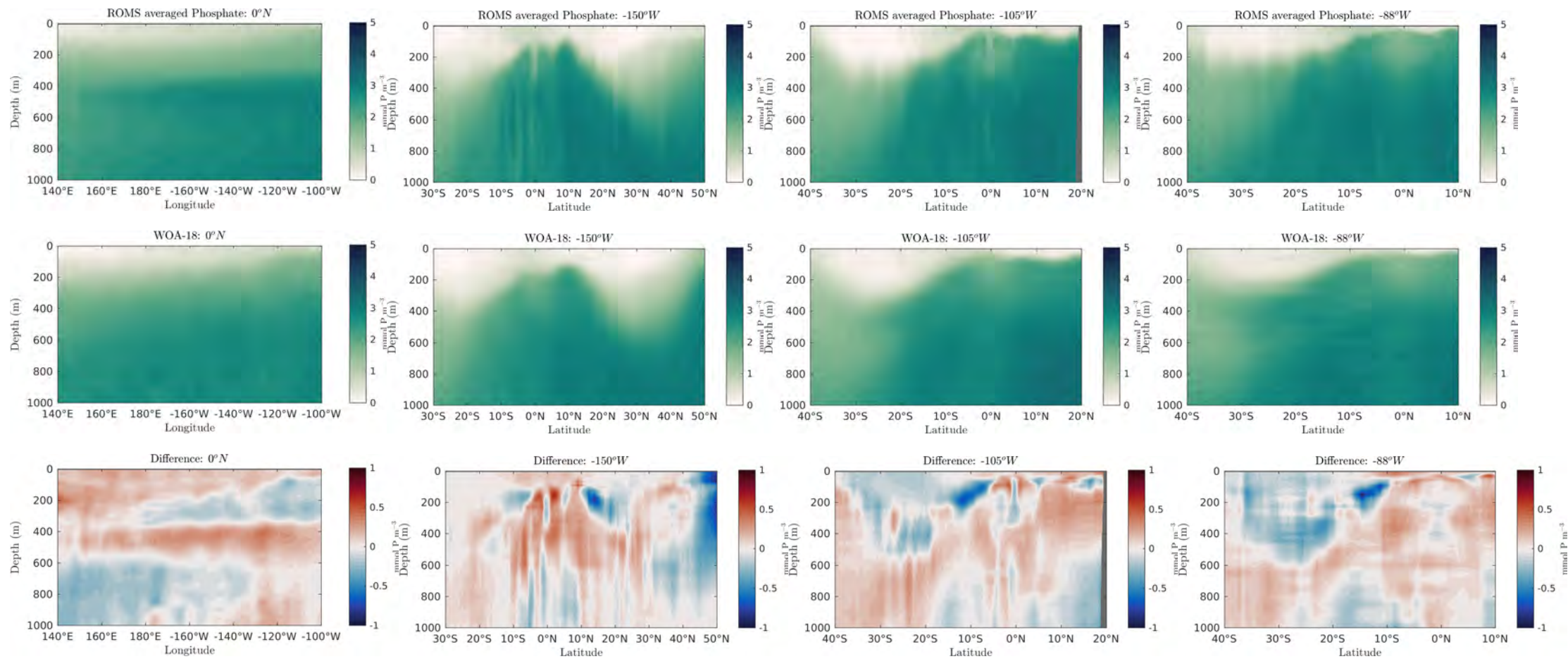
Figure 29: Phosphate transects
