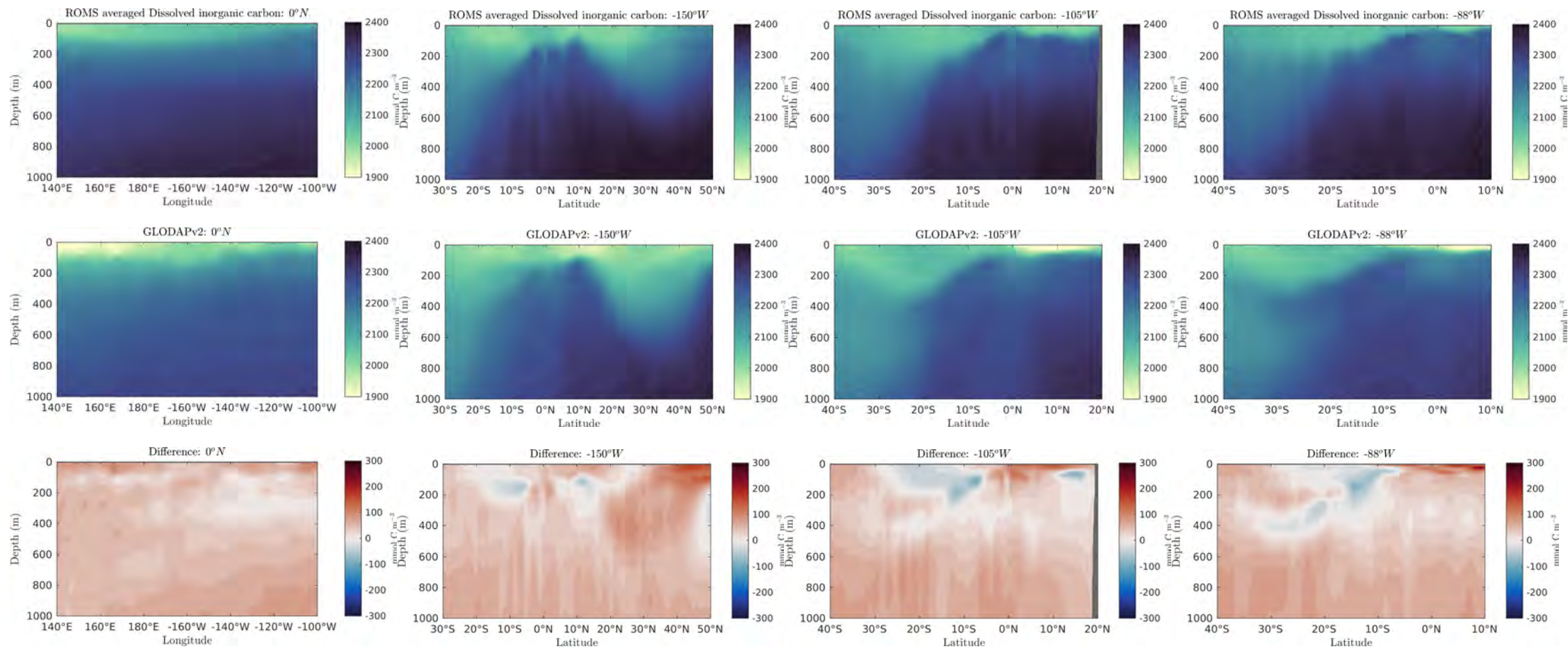
Figure 38: DIC transects
