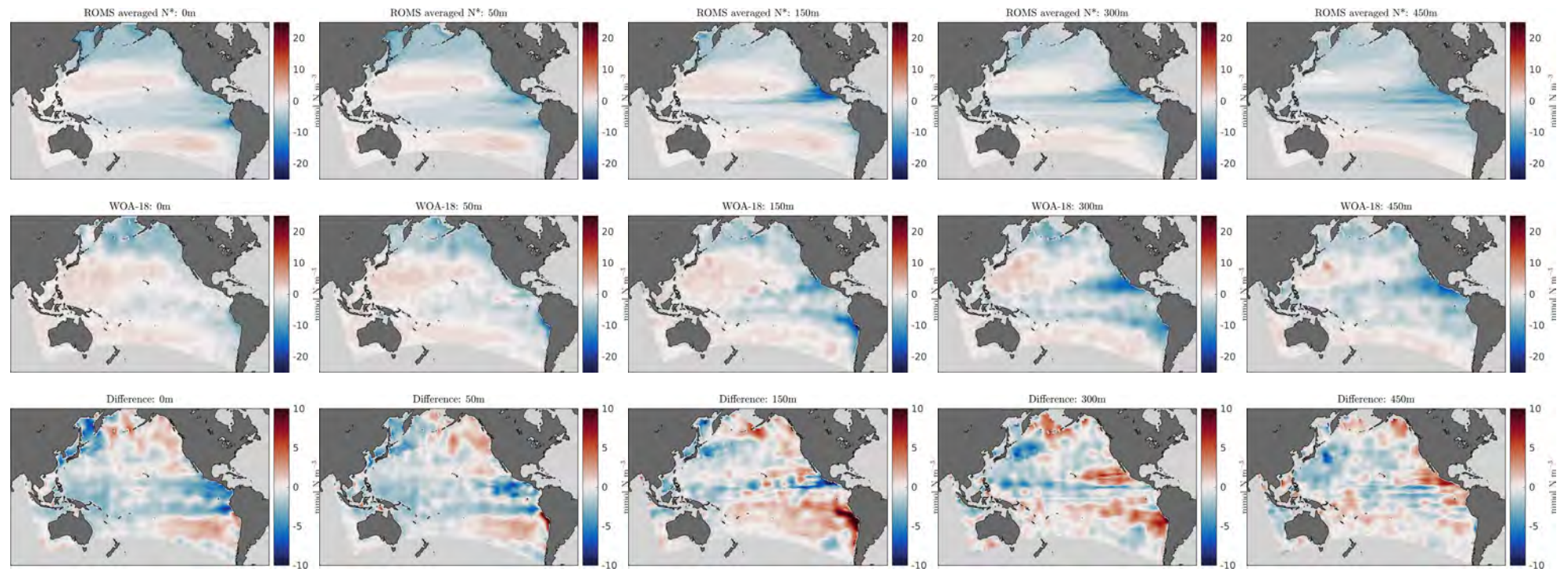
Figure 14: N^* Z-Slices
