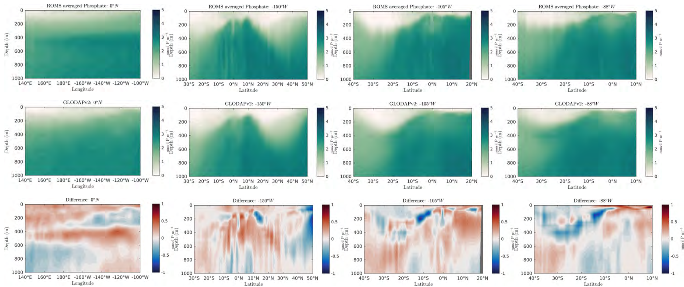
Figure 30: Phosphate transects
