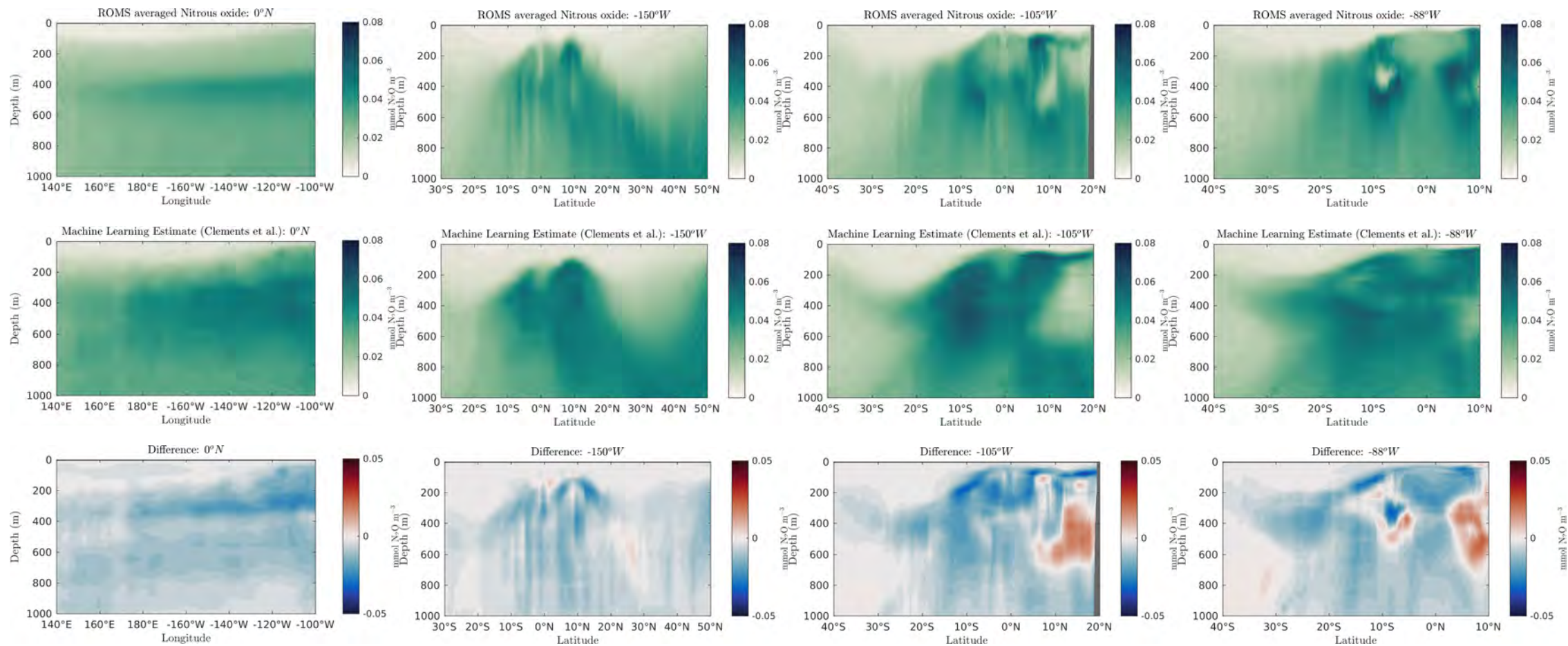
Figure 32: Nitrous Oxide transects
