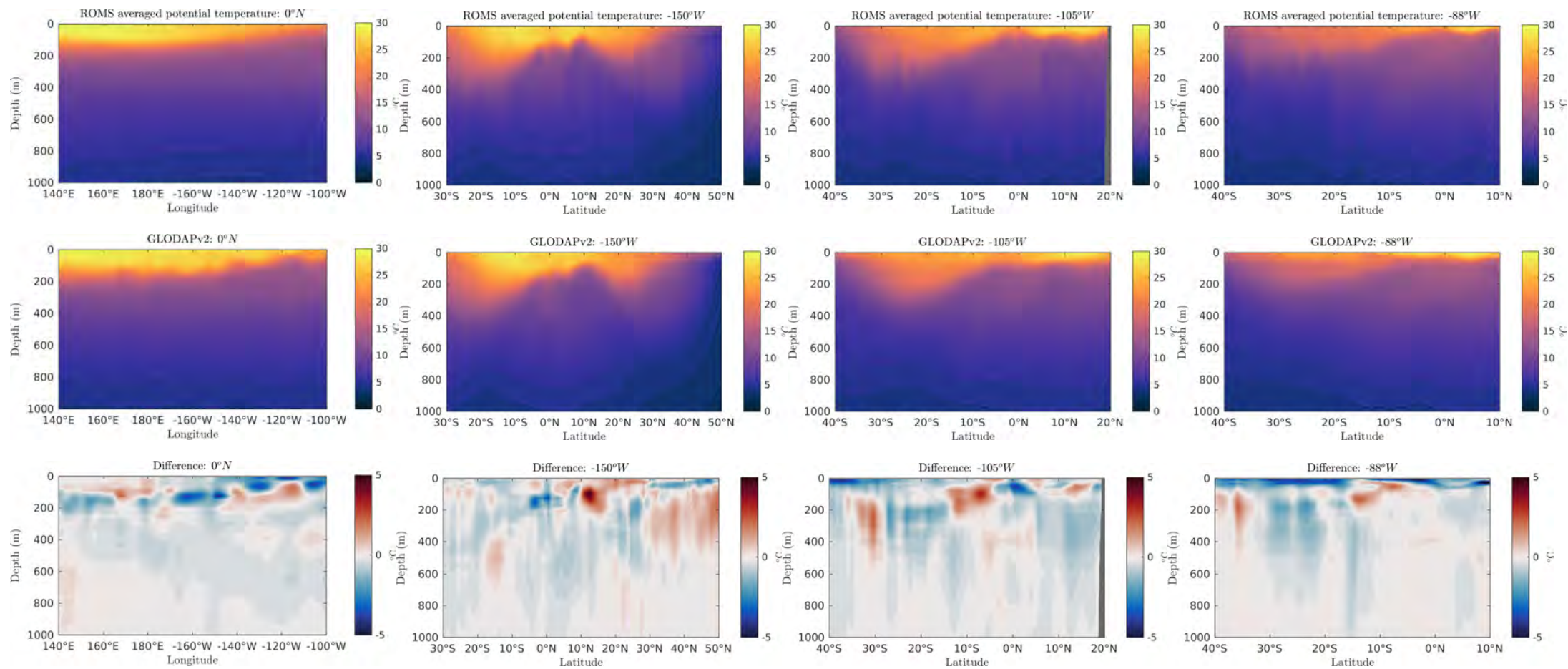
Figure 22: Temperature transects
