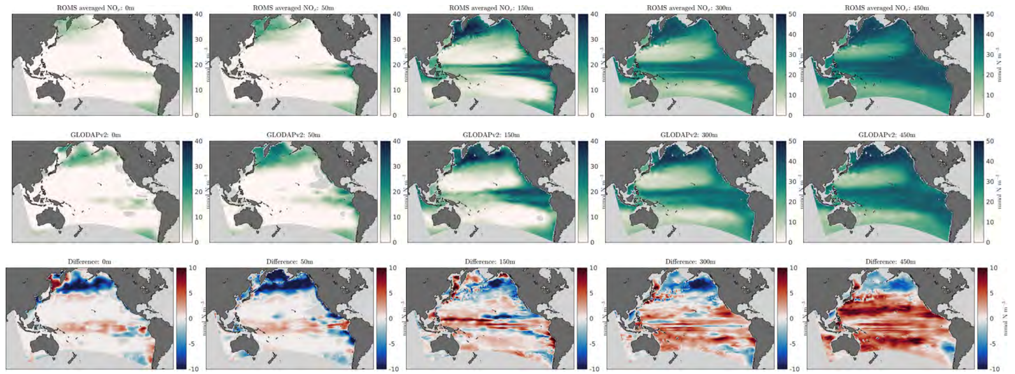
Figure 8: Nitrate+Nitrite Z-Slices
