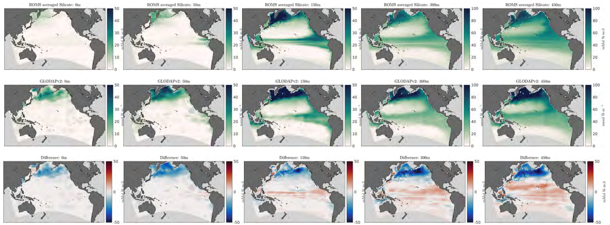
Figure 17: Silicate Z-Slices
