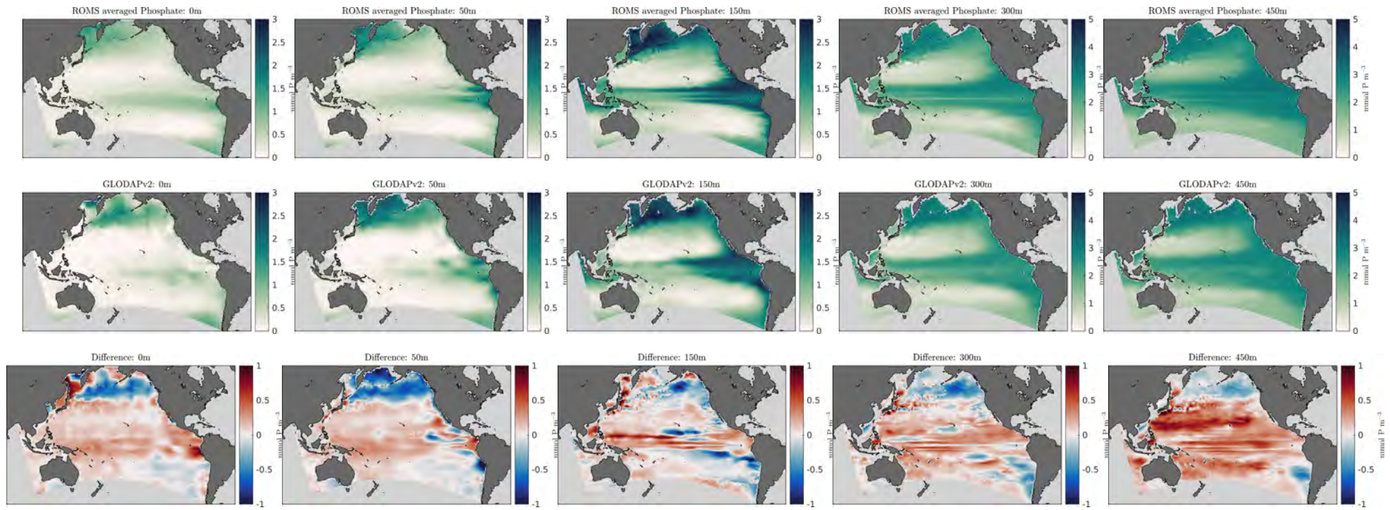
Figure 10: Phosphate Z-Slices
