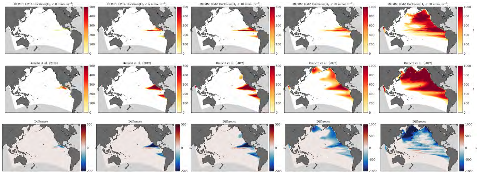
Figure 48: OMZ Thickness
