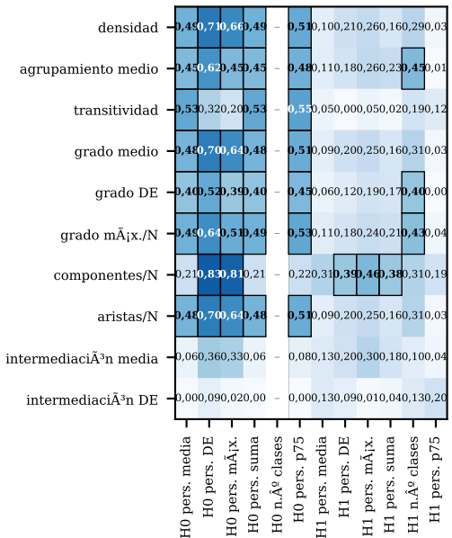
CIFAR-10
