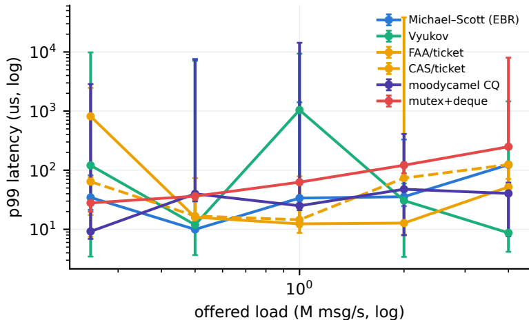
schedule-to-dequeue latency; exact sample-count rows
