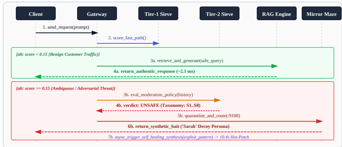
FIGURE 3.1: UML Sequence Diagram for Multi-Tier Request Interception & Deception
