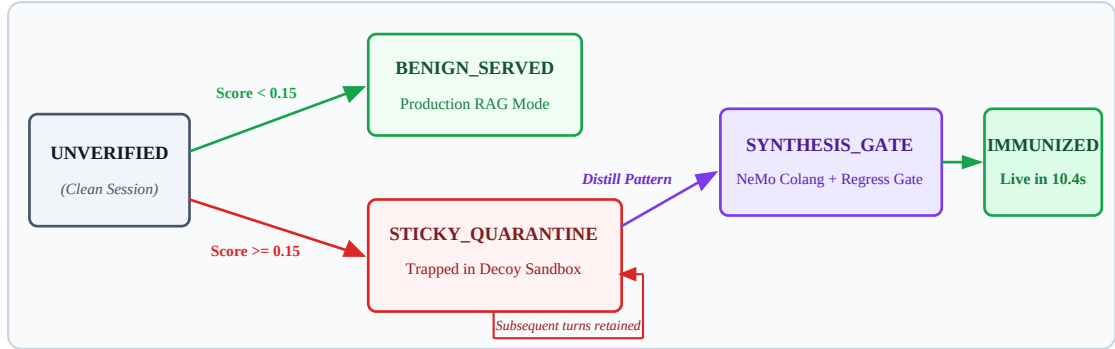
FIGURE 4.1: UML State Machine Diagram for Session Quarantine & Self-Healing Loop
