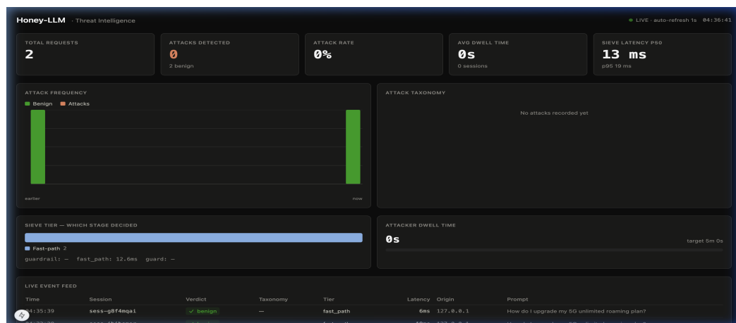
FIGURE 4.4: Dark SOC Real-Time Threat Intelligence Dashboard (/dashboard)
