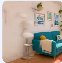
Probe: \hat{x}_{0,i}(\tau^*)
