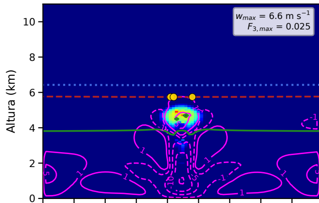
(a) CTRL t \approx 20 min
