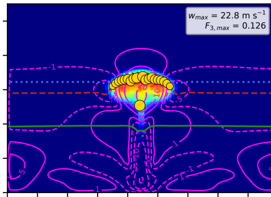
(b) DYN_PLUS t \approx 20 min
