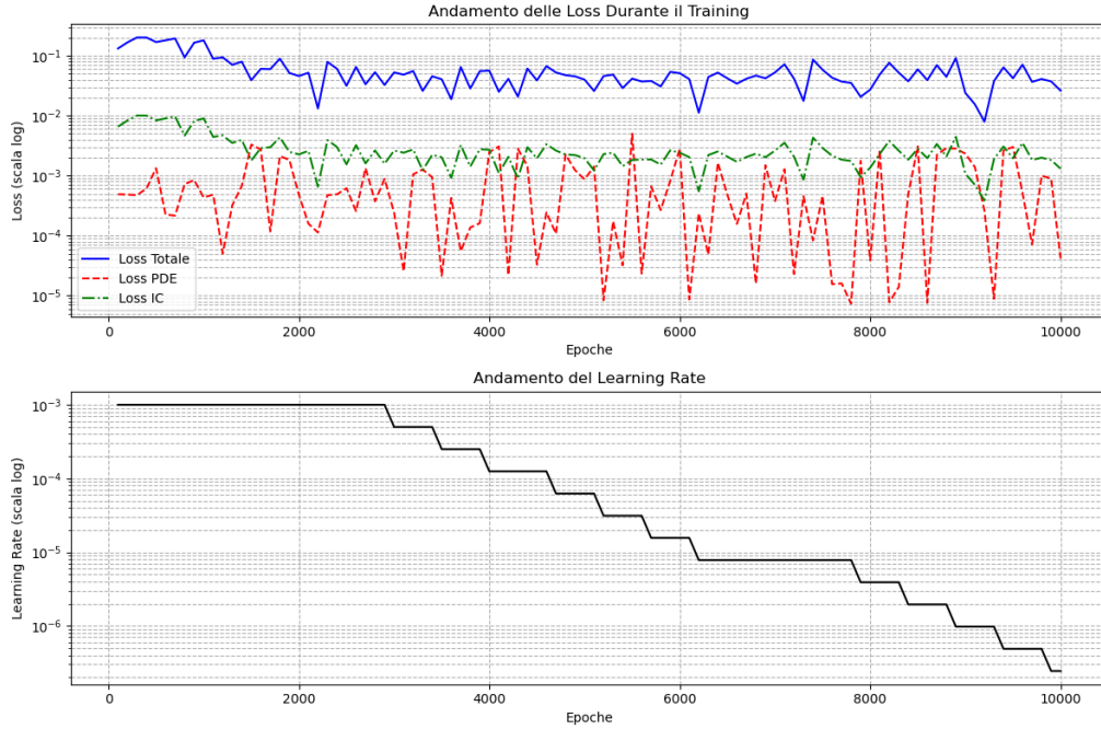
Figure 8: Training loss for the PINN model ( pinn_{model_13908} ).
