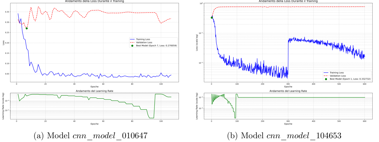
Figure 6: Training losses for CNNs with advanced regularization techniques.
