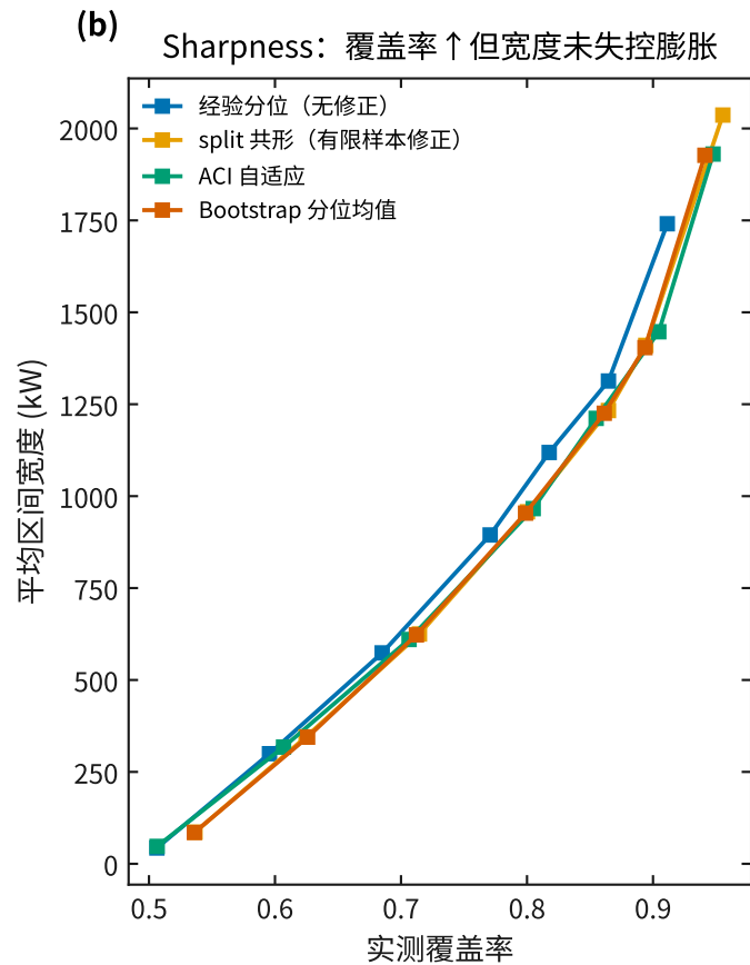
Fig.4 Q2 概率标定与经济权衡: Reliability / Sharpness / Cost-Risk
