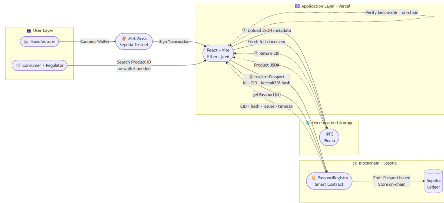
Fig. 1. EcoPassEU system architecture.
