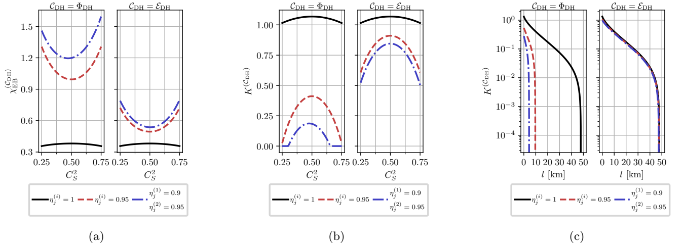
Figure 5: (a) Holevo information, \chi_{EB}^{(C_{DH})} , and (b) asymptotic secret fraction, K^{(C_{DH})} , as functions of the signal beam-splitter transmittance C_S^2 , computed for the additive-noise and attenuator channels at the detector efficiencies specified in the subfigure titles. The parameters are V = 5 , T_{ch} = 0.95 , \xi_{ch} = 10^{-2} , and \beta = 0.95 . (c) K^{(C_{DH})} versus channel length l for the two channels. The parameters are V = 5 , \beta = 0.95 , and \xi_{ch} = 10^{-2} ; the fiber attenuation is 20 dB per 100 km. For both channels, r = (r_2 + r_1)/2 . The beam splitters in the two homodyne branches are balanced, and detector efficiencies not specified in the subfigure titles are set to unity.
