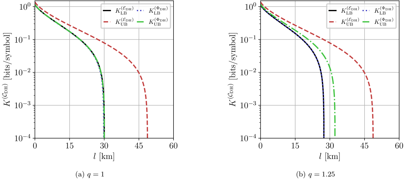
Figure 4: Asymptotic secret fraction K^{(C_{DH})} versus channel length l , computed for fixed \sigma_x^{(i)} = 1.01 (see Eq.(18)) and various imbalance ratios q \equiv \frac{S_S^2}{C_S^2} (17) for additive-noise and attenuator channel models (see Fig. 3). The parameters are: V = 5 ; \beta = 0.95 ; \xi_{ch} = 10^{-2} ; the fiber loss is 20 dB per 100 km.
