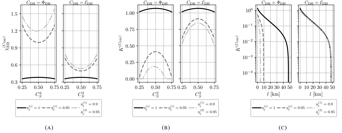
FIG. 5. (a) Holevo information, \chi_{EB}^{(C_{DH})} and (b) asymptotic secret fraction, K^{(C_{DH})} , as a function of the signal beam splitter transmission, C_S^2 , of the double homodyne receiver computed at different values of the detector efficiencies for additive noise and attenuator channel models, as indicated in panel title. The parameters are: V = 5 ; T_{ch} = 0.95 ; \xi_{ch} = 10^{-2} ; and \beta = 0.95 . (c) K^{(C_{DH})} versus transmission length l for additive noise and attenuator channel models. The parameters are: V = 5 ; \beta = 0.95 ; \xi_{ch} = 10^{-2} ; losses are 20 dB per 100 km.. For both channel models r = \frac{r_2 + r_1}{2} (see main text).
