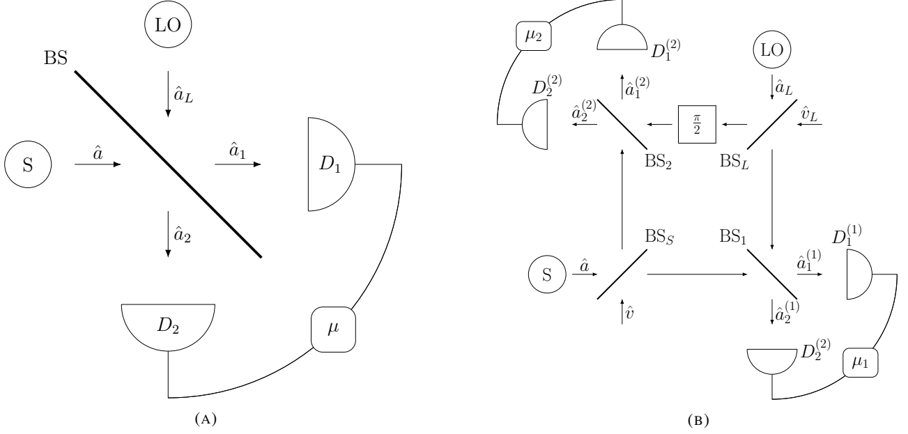
FIG. 1. (a) Scheme of homodyne receiver. S (LO) is the source of signal (reference) mode, BS is the beamsplitter with transmission and reflection coefficients C and S , respectively; photodetectors D_1 and D_2 have quantum efficiencies \eta_1 and \eta_2 , and \mu = m_1 - m_2 is the photon count difference. (b) Scheme of double homodyne receiver. S (LO) is the source of signal (reference) mode, BS_S ( BS_L ) is the signal mode (local oscillator) beam splitter; \frac{\pi}{2} is the quarter wave phase shifter; BS_i is the beam splitter of i th homodyne; D_{1,2}^{(i)} are the photodetectors of the i th homodyne; and \mu_i = m_1^{(i)} - m_2^{(i)} is the photon count difference registered by the detectors of i th homodyne.
