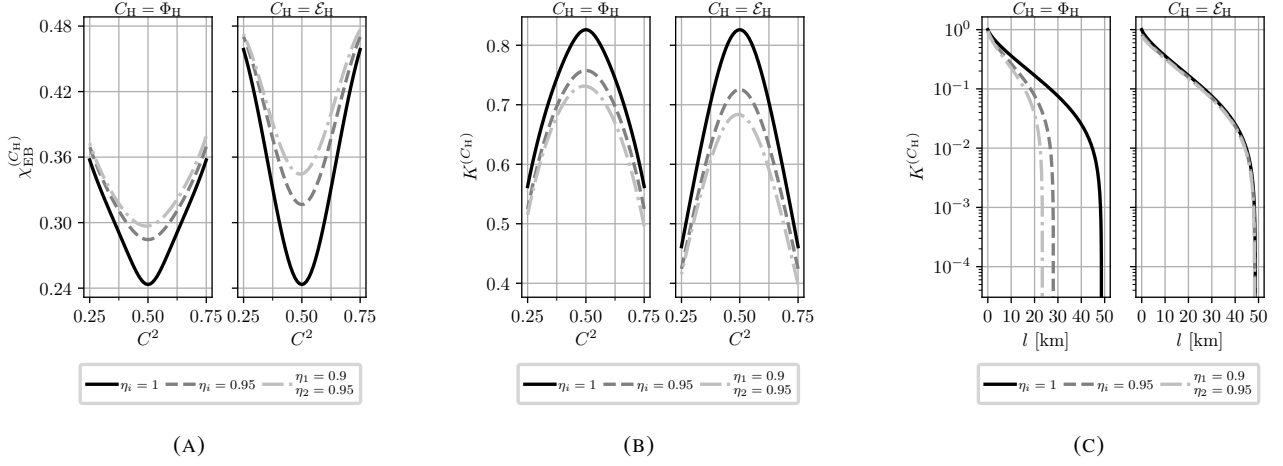
FIG. 2. (a) Holevo information, \chi_{EB}^{(C_H)} and (b) asymptotic secret fraction, K^{(C_H)} , as a function of the beam splitter transmission, C^2 , of the homodyne receiver computed at different values of the detector efficiencies for additive noise and attenuator channel models, as indicated in panel title. The parameters are: V = 5 ; T_{ch} = 0.95 ; \xi_{ch} = 10^{-2} ; and \beta = 0.95 . (c) K^{(C_H)} versus transmission length l for additive noise and attenuator channel models. The parameters are: V = 5 ; \beta = 0.95 ; \xi_{ch} = 10^{-2} ; losses are 20 dB per 100 km.
