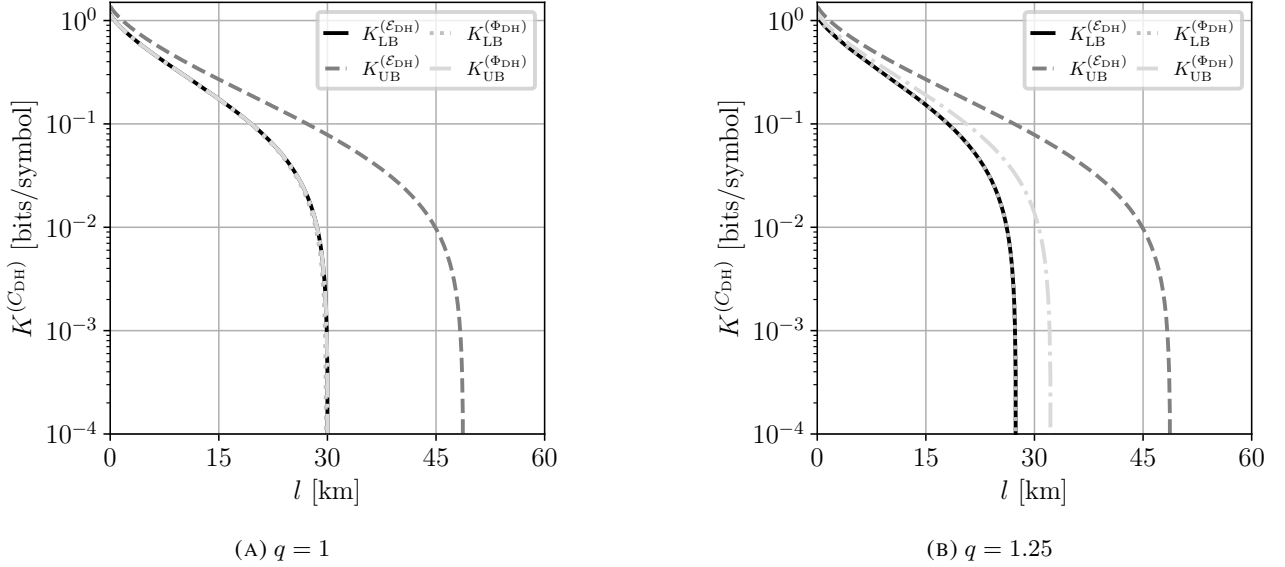
FIG. 4. Asymptotic secret fraction K^{(C_{DH})} versus channel length l , computed for fixed \sigma_x^{(i)} = 1.05 (see Eq.(14)) and various imbalance ratios q \equiv \frac{S_S^2}{C_S^2} for additive noise and attenuator channel models (see Fig. 3). The parameters are: V = 5 ; \beta = 0.95 ; \xi_{ch} = 10^{-2} ; losses are 20 dB per 100 km.
