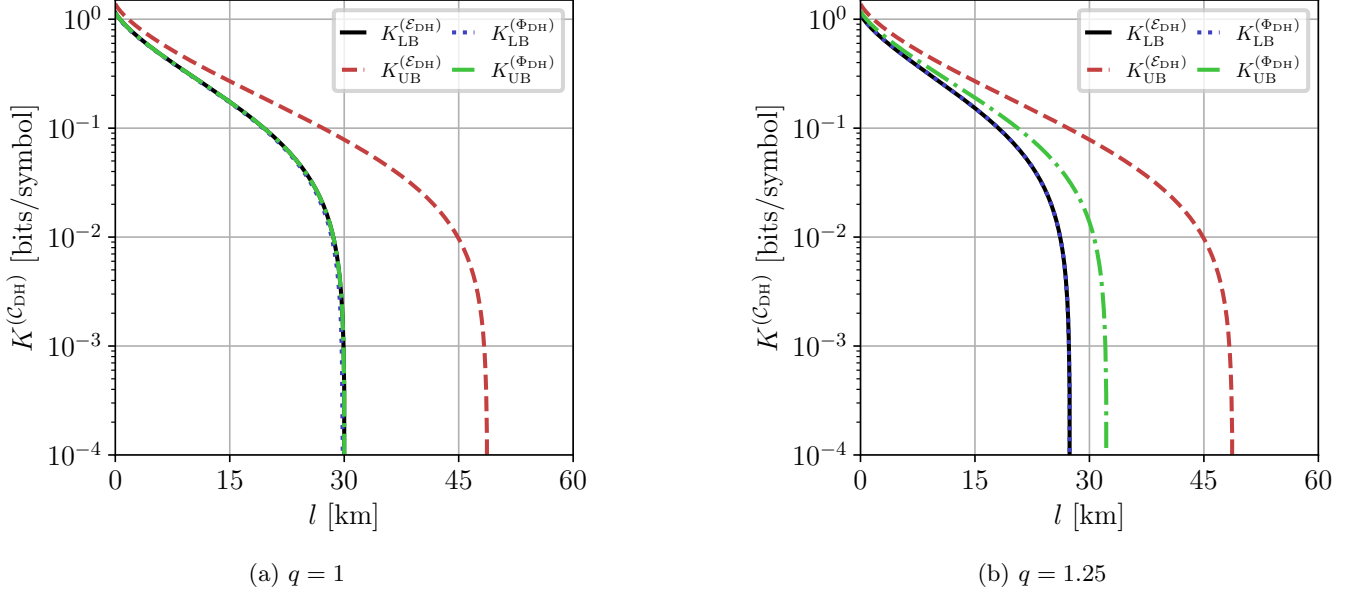
Figure 4: Asymptotic secret fraction K^{(C_{DH})} versus channel length l , computed for fixed \sigma_x^{(i)} = 1.05 (see Eq.(14)) and various imbalance ratios q \equiv \frac{S_S^2}{C_S^2} for additive-noise and attenuator channel models (see Fig. 3). The parameters are: V = 5 ; \beta = 0.95 ; \xi_{ch} = 10^{-2} ; losses are 20 dB per 100 km.
