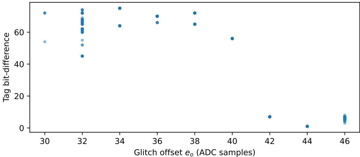
Fault band structure: tag differential vs glitch offset
