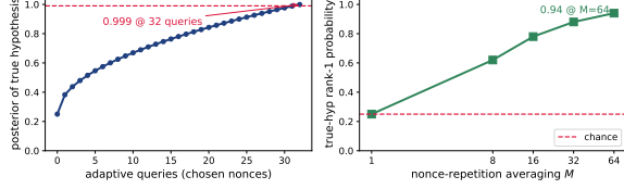
Fig. 2. (a) Closed-loop adaptive attack: posterior on correct 2 key bits reaches 0.999 in 32 queries. (b) Trace averaging ( M ): rank-1 probability rises from 0.25 to 0.94 at M=64 .
