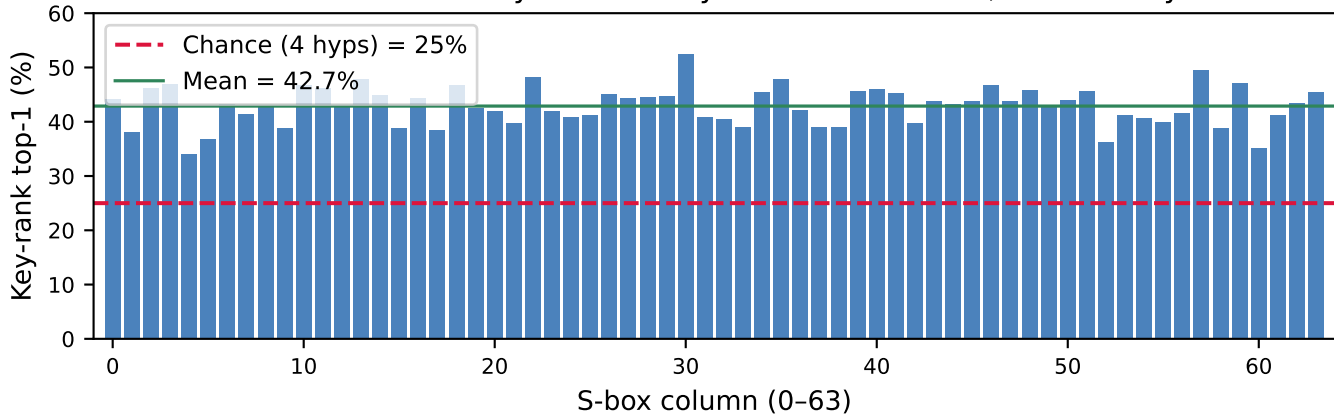
Per-column CNN key-bit recovery — held-out traces, random keys
