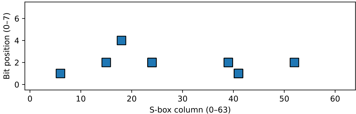
Localized single-bit faults at round-11 S-box input
