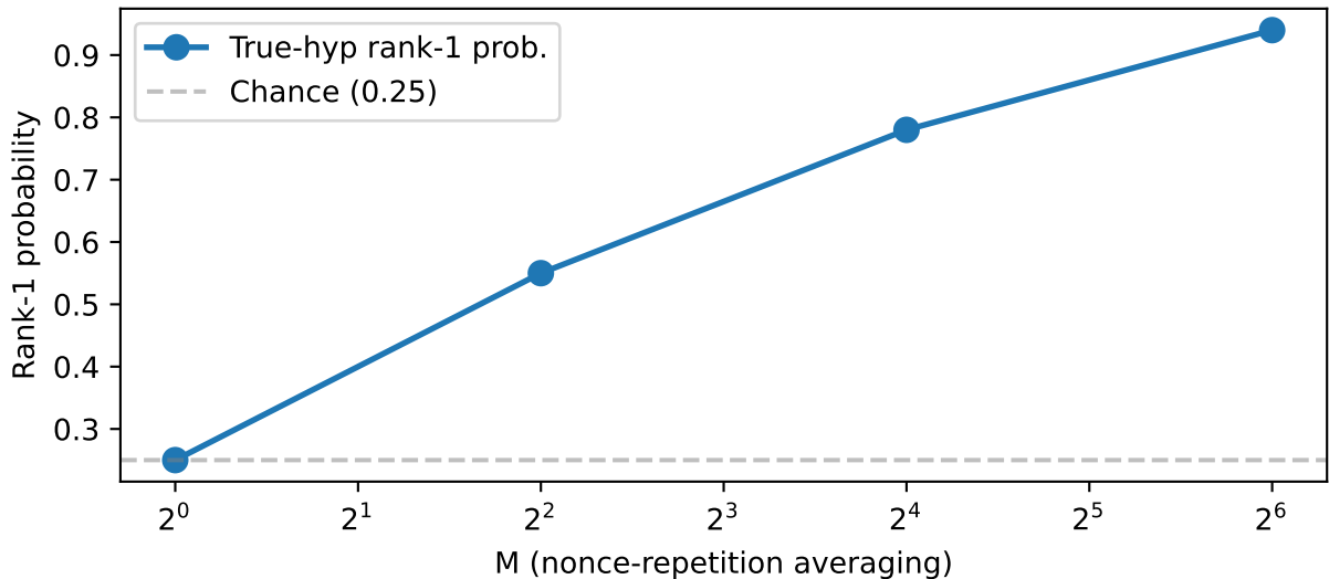
M-averaging as SNR lever (measured on hardware)
