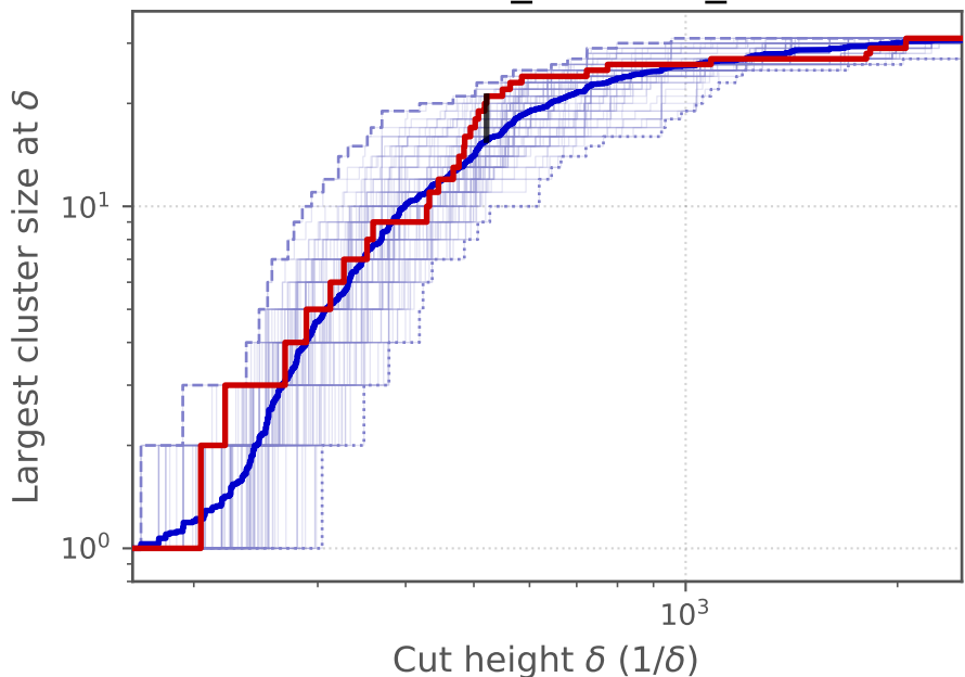
Cluster sizes across hierarchy cuts for network_1 scores_2
