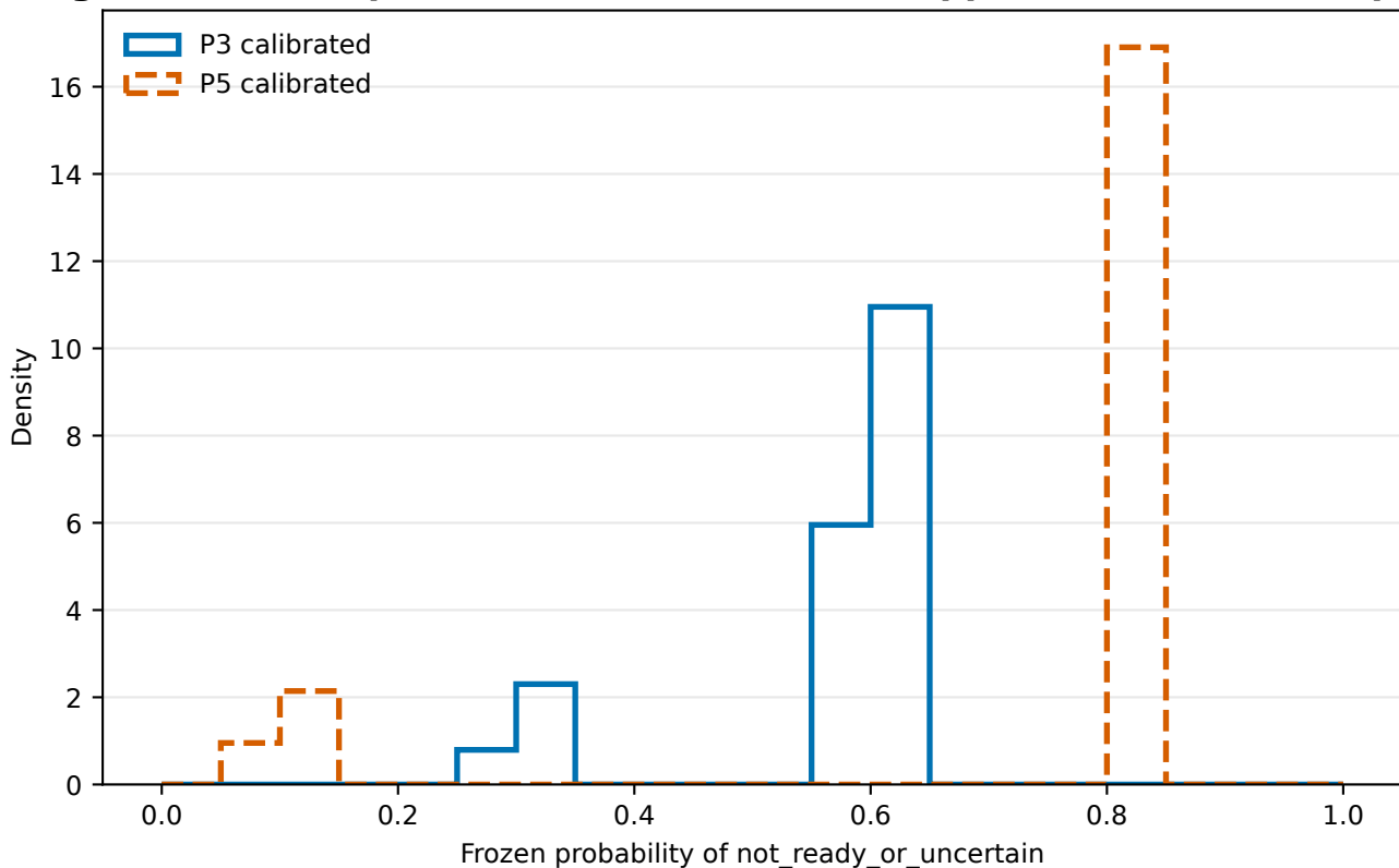
Figure 5. Frozen prediction distributions in supported confirmation pairs
