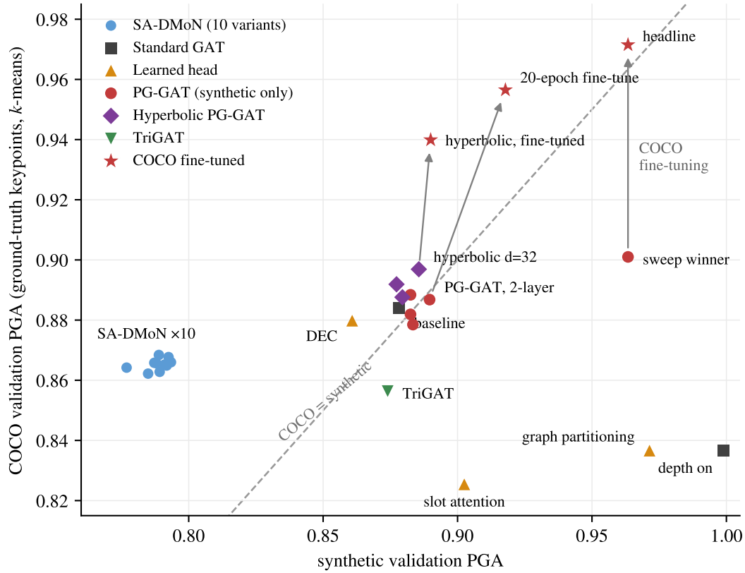
Figure 5.1. Synthetic-validation PGA against COCO-validation PGA using ground-truth keypoints and k -means for the 27 configurations in Chapter 4 that report both metrics. The dashed diagonal represents equal performance on the two datasets; points below it perform worse on COCO than on the synthetic validation set, with the vertical distance from the diagonal indicating the transfer gap. Arrows connect the three synthetic-only models to their corresponding COCO fine-tuned versions, showing the change produced by real-data adaptation. Values are taken directly from the results reported in Chapter 4. TriGAT is evaluated on the 2,180 scenes containing valid triplets, while all other configurations are evaluated on 2,307 scenes.
