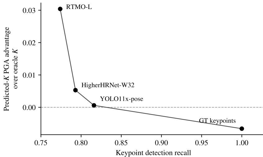
Figure 5.2. Difference in PGA between predicted- K and oracle- K grouping as a function of keypoint recall for the three detector evaluations and the ground-truth-keypoint control. The predicted- K advantage increases across the three detector operating points as recall decreases, while the ground-truth-keypoint control reverses the effect when the input is complete. This pattern is consistent with the effective-person-count explanation - annotation-level K becomes a less appropriate clustering constraint as the detected keypoint set becomes less complete.
