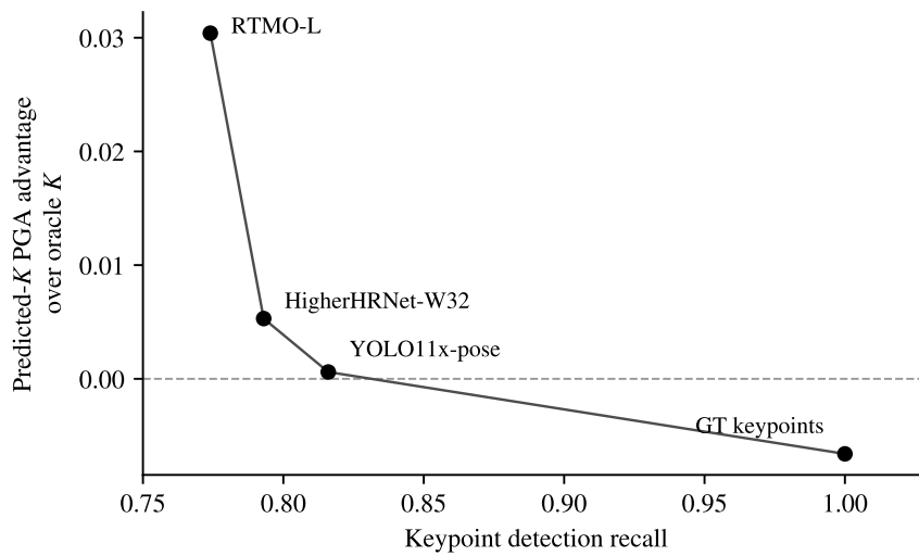
Figure 5.3. Difference in PGA between predicted- K and oracle- K grouping as a function of keypoint recall for the three detector evaluations and the ground-truth-keypoint control. The predicted- K advantage increases across the three detector operating points as recall decreases, while the ground-truth-keypoint control reverses the effect when the input is complete. This pattern is consistent with the effective-person-count explanation - annotation-level K becomes a less appropriate clustering constraint as the detected keypoint set becomes less complete.
