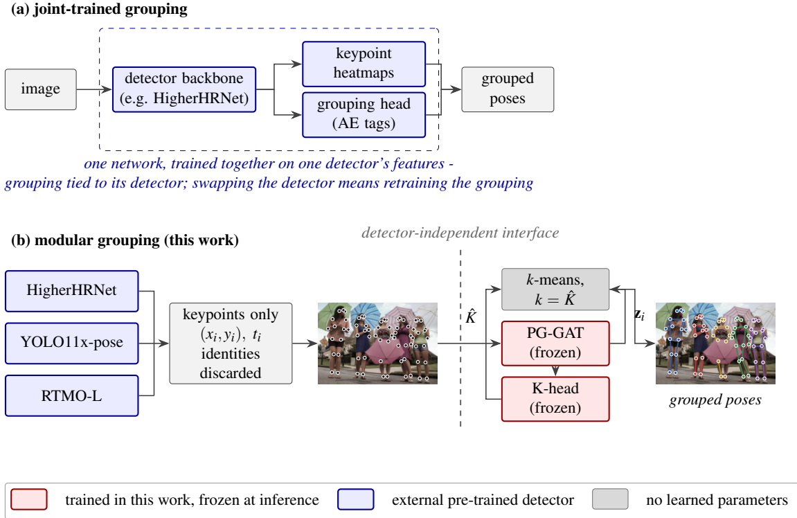
Figure 1.2. Joint-trained grouping compared with the modular grouping pipeline developed in this work. (a) In established bottom-up methods, the grouping head is trained jointly with the keypoint detector and operates on detector-specific features, coupling the grouping mechanism to that detector. (b) The modular pipeline instead exposes a keypoint-only interface shared by all three evaluated detectors. PG-GAT embeds the detected keypoints, the K-head estimates the number of people \hat{K} , and k -means partitions the embeddings into person groups. PG-GAT and the K-head are trained once and remain frozen when the upstream detector is changed. The insets show COCO val2017 image 281759 using pooled HigherHRNet detections before grouping (grey) and after grouping by the modular pipeline (coloured by person). Red blocks denote components trained in this work and frozen at inference, blue blocks denote external pre-trained detectors, and grey blocks contain no learned parameters.
