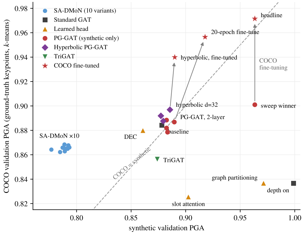
Figure 5.2. Synthetic-validation PGA against COCO-validation PGA using ground-truth keypoints and k -means for the 27 configurations in Chapter 4 that report both metrics. The dashed diagonal represents equal performance on the two datasets; points below it perform worse on COCO than on the synthetic validation set, with the vertical distance from the diagonal indicating the transfer gap. Arrows connect the three synthetic-only models to their corresponding COCO fine-tuned versions, showing the change produced by real-data adaptation. Values are taken directly from the results reported in Chapter 4. TriGAT is evaluated on the 2,180 scenes containing valid triplets, while all other configurations are evaluated on 2,307 scenes.
