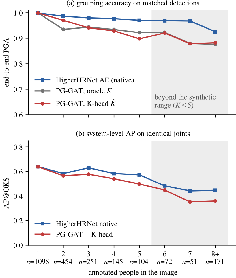
Figure B.2. End-to-end PGA and AP@OKS against the number of annotated people in each image using HigherHRNet detections. (a) PGA on the matched detections of the 2,165 scored scenes from Section 4.9, comparing HigherHRNet’s native associative-embedding grouping, PG-GAT using the annotated K , and PG-GAT using the K -head prediction \hat{K} . (b) AP@OKS over all 5,000 COCO val2017 images for the native grouping and autonomous PG-GAT pipeline using the same pooled joints, evaluated separately within each person-count bin using the COCO evaluator. The final bin contains images with eight or more annotated people, the shaded region marks counts beyond the K \leq 5 range used during synthetic training, and n gives the number of images in each AP bin.
