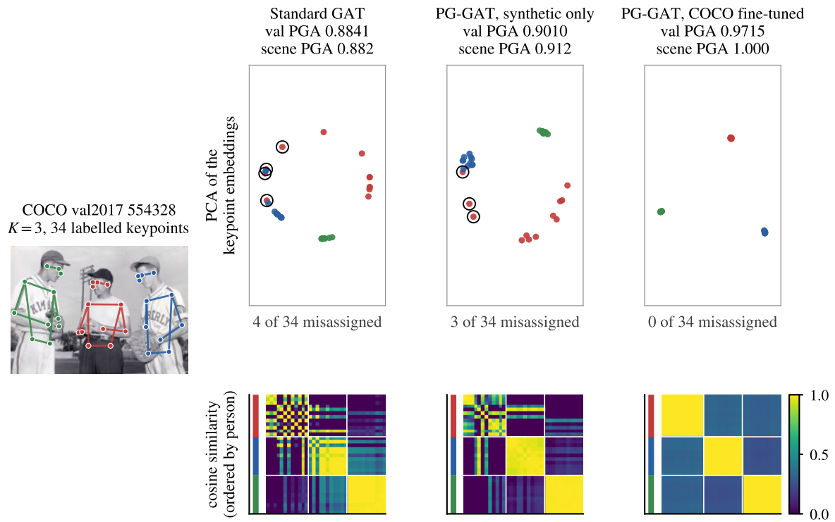
Figure B.1. Per-keypoint embeddings of COCO val2017 image 554328 ( K=3 , 34 labelled keypoints) under the standard GAT baseline (run jdk11n4a ), the synthetic-only PG-GAT ( 08d0ffde ), and the COCO fine-tuned headline PG-GAT ( b5noyg7t ). The top row shows the first two principal components of the embeddings, coloured by ground-truth person; keypoints assigned to the wrong person by the k -means read-out are ringed. The corresponding per-scene PGA values are 0.882, 0.912, and 1.000. The bottom row shows the cosine-similarity matrices of the same embeddings, with keypoints ordered by ground-truth person.
