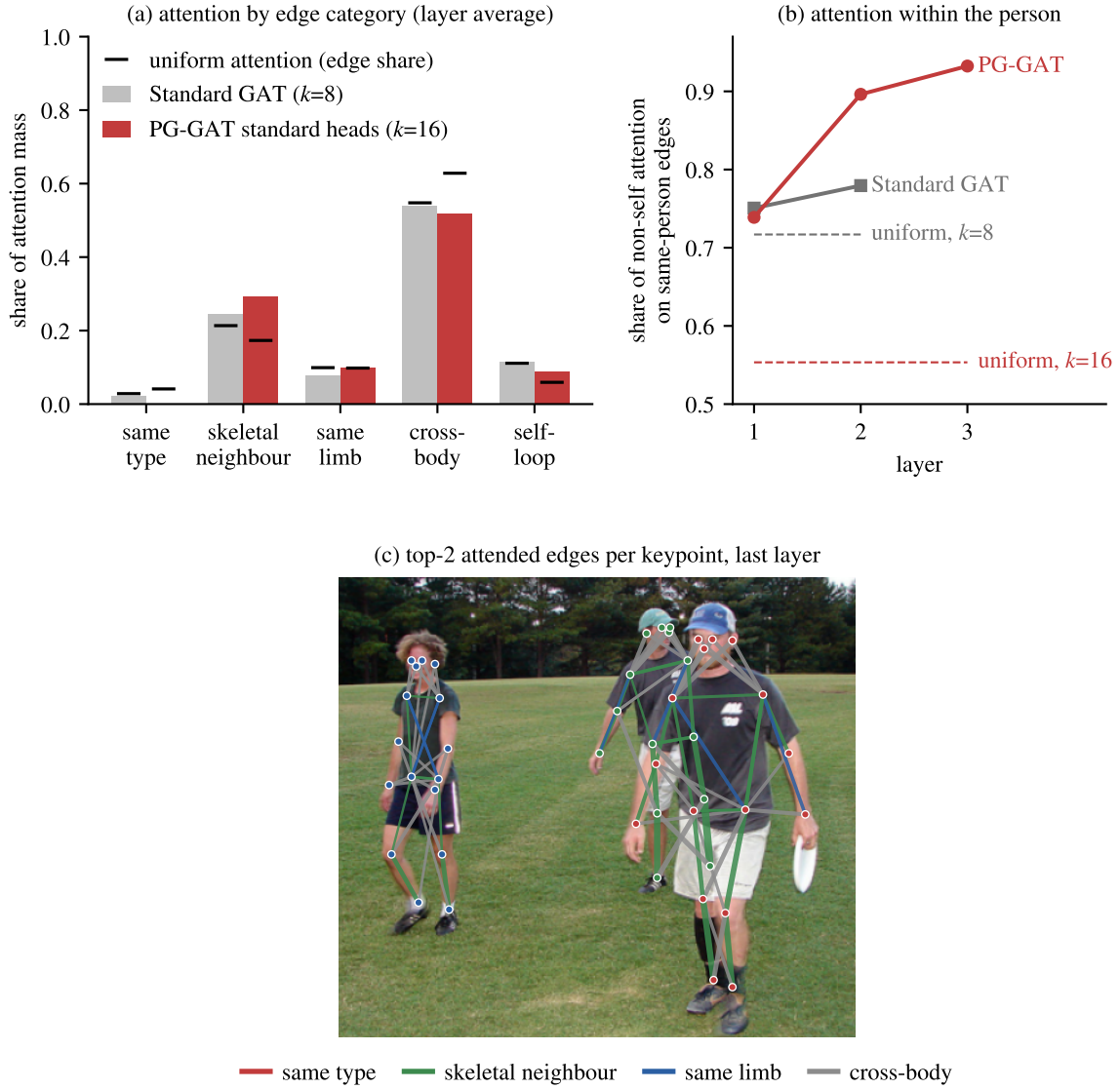
Figure 5.1. GATv2 attention measured on the 1,248 multi-person COCO val2017 scenes using ground-truth keypoints. (a) Share of attention mass by edge category for the standard GAT baseline and the PG-GAT standard heads, averaged across layers and heads. Black markers show the corresponding share under uniform attention, given by the fraction of edges belonging to each category. The self-loop is added to each node by GATv2Conv. (b) Per-layer share of non-self attention assigned to same-person edges, compared with the corresponding uniform share. (c) The two highest-attention incoming edges for each keypoint in the final PG-GAT layer on COCO image 482800 (the scene shown in Figure 1.1), coloured by edge category and drawn with width proportional to their attention coefficient. Attention coefficients are recorded by wrapping the attention layers during inference without modifying either trained model.
