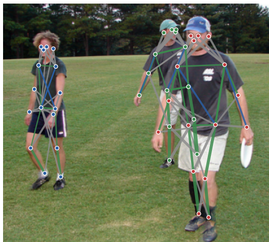
(c) top-2 attended edges per keypoint, last layer
