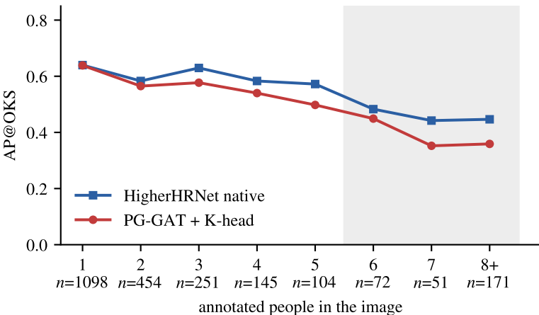
(b) system-level AP on identical joints
