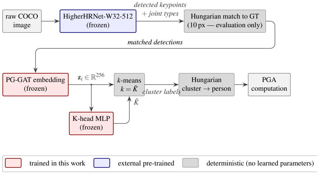
Figure 3.4. The autonomous end-to-end pose-grouping pipeline. HigherHRNet detects candidate keypoints and assigns each a joint type. The frozen PG-GAT network embeds the resulting detection set, the frozen K-head MLP predicts the number of people \hat{K} , and k -means with k = \hat{K} produces the final per-person partition. Hungarian matching to ground-truth keypoints is performed only after inference to associate matched detections with person identifiers for PGA evaluation - it is not an input to the grouping pipeline. Components trained in this work and frozen at inference (PG-GAT and the K-head) are shown in red, the external pre-trained detector in blue, and deterministic operations with no learned parameters ( k -means and evaluation-only Hungarian matching) in grey.
