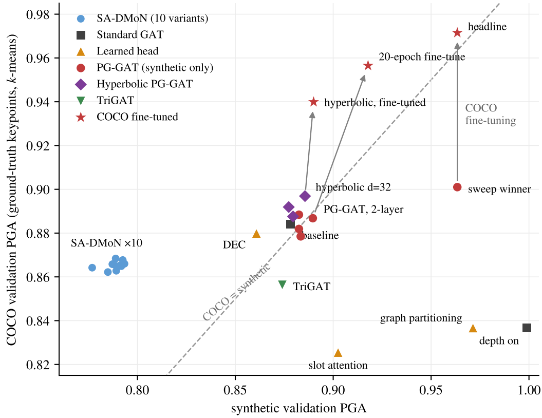
Figure 5.1. Synthetic-validation PGA against COCO-validation PGA (ground-truth keypoints, k -means) for the 27 configurations of Chapter 4 that report both. Points below the dashed diagonal lose accuracy in transfer; the vertical distance to the diagonal is the transfer gap. Arrows join the three synthetic-only models to their COCO fine-tuned versions. Values are the Chapter 4 table cells - TriGAT is scored on 2,180 scenes, every other configuration on 2,307.
