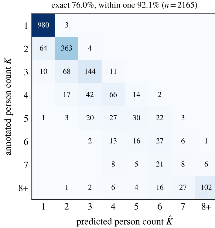
Figure 4.3. Predicted person count \hat{K} from the frozen K head against the annotated count K on the 2,165 scored HigherHRNet scenes. Counts of eight or more are pooled into the last row and column. Mass below the diagonal is under-counting. The matrix comes from a re-run of the pipeline that reproduces the reported aggregates to within 0.0003 PGA; two scenes receive a different count than in the logged run, which is why the exact-count rate reads 76.0% here against 76.1% in the text.
