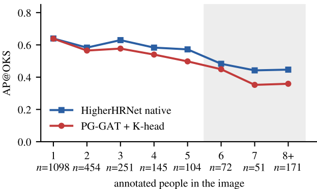
(b) system-level AP on identical joints
