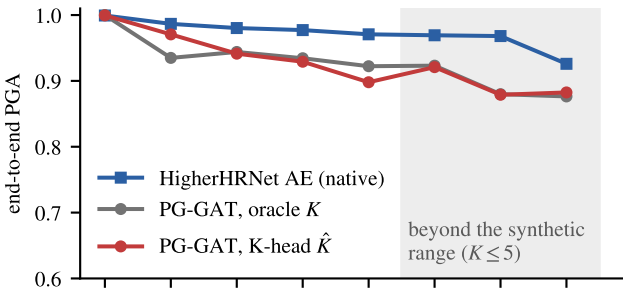
(a) grouping accuracy on matched detections
