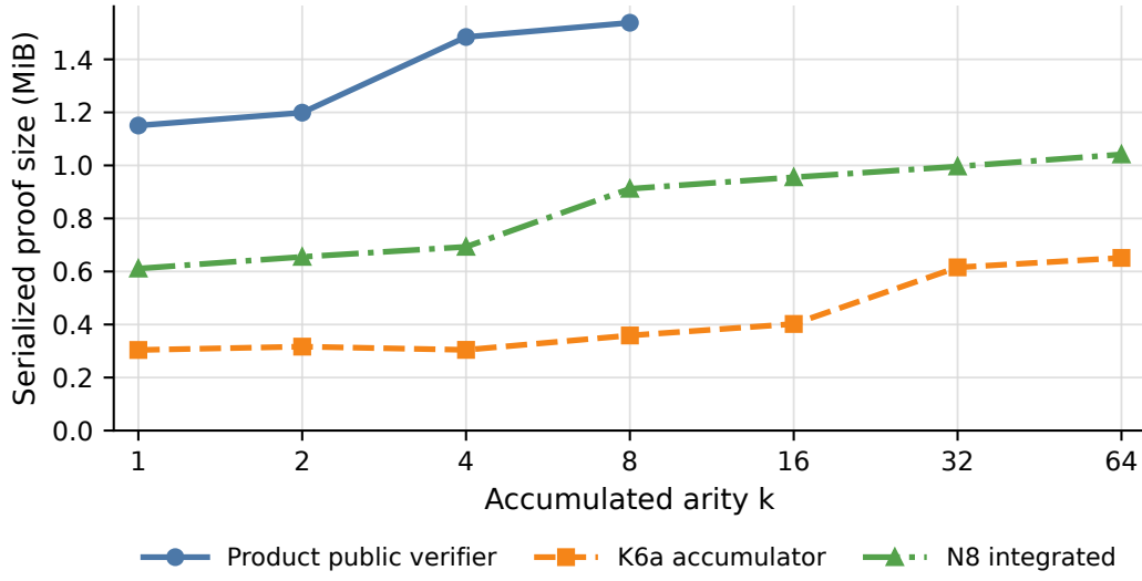
Figure 4: Serialized proof size versus arity. The accumulator routes keep a single public transition proof shape rather than a list of independent WHIR proofs.
