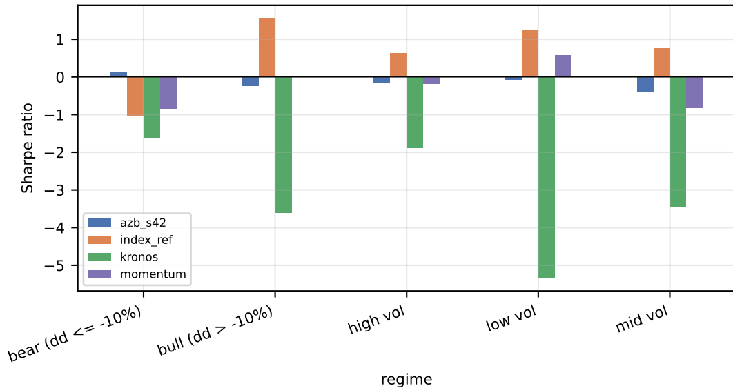
Performance by prespecified regime (baseline costs)
