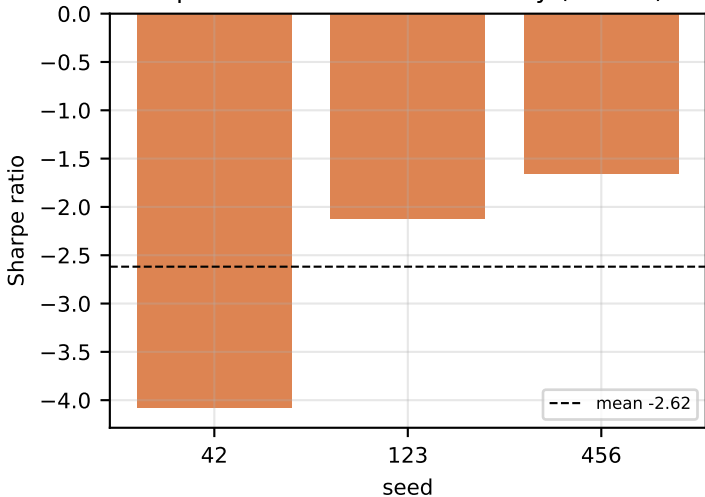
AlphaZeroBeta seed sensitivity (3 folds)
