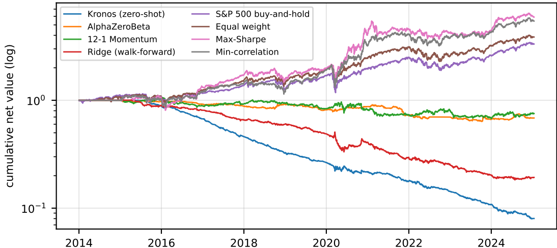
Out-of-sample equity curves, S&P 500, 22 walk-forward folds (baseline costs)
