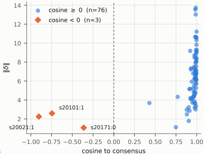
(b) Held-out streams: direction vs magnitude
