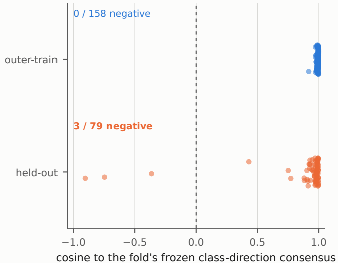
(a) Class-direction coherence, B0
