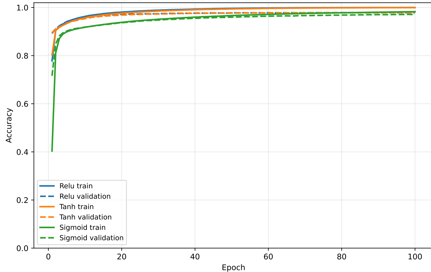
H3: Accuracy by Activation Function
