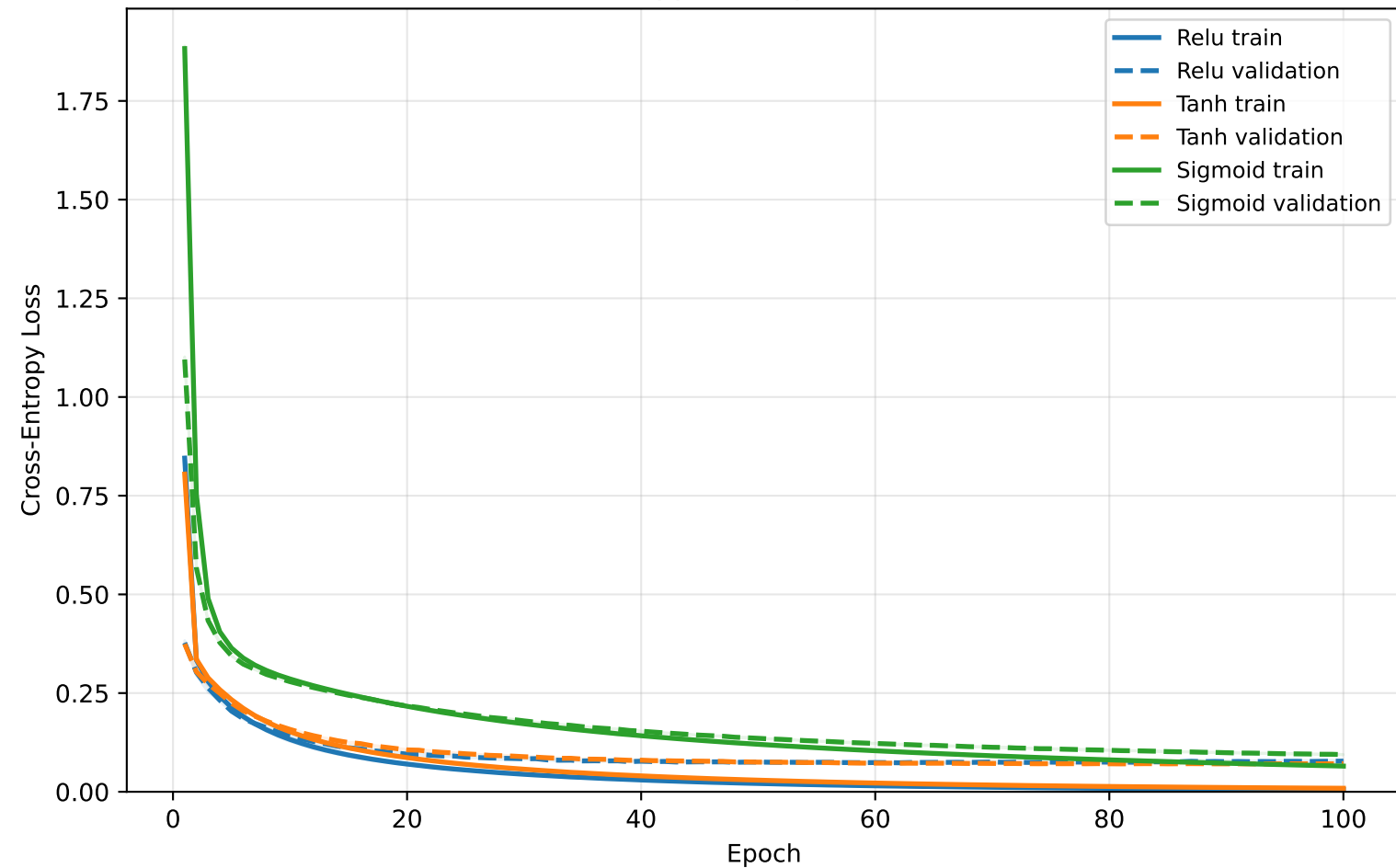
H3: Cross-Entropy Loss by Activation Function
