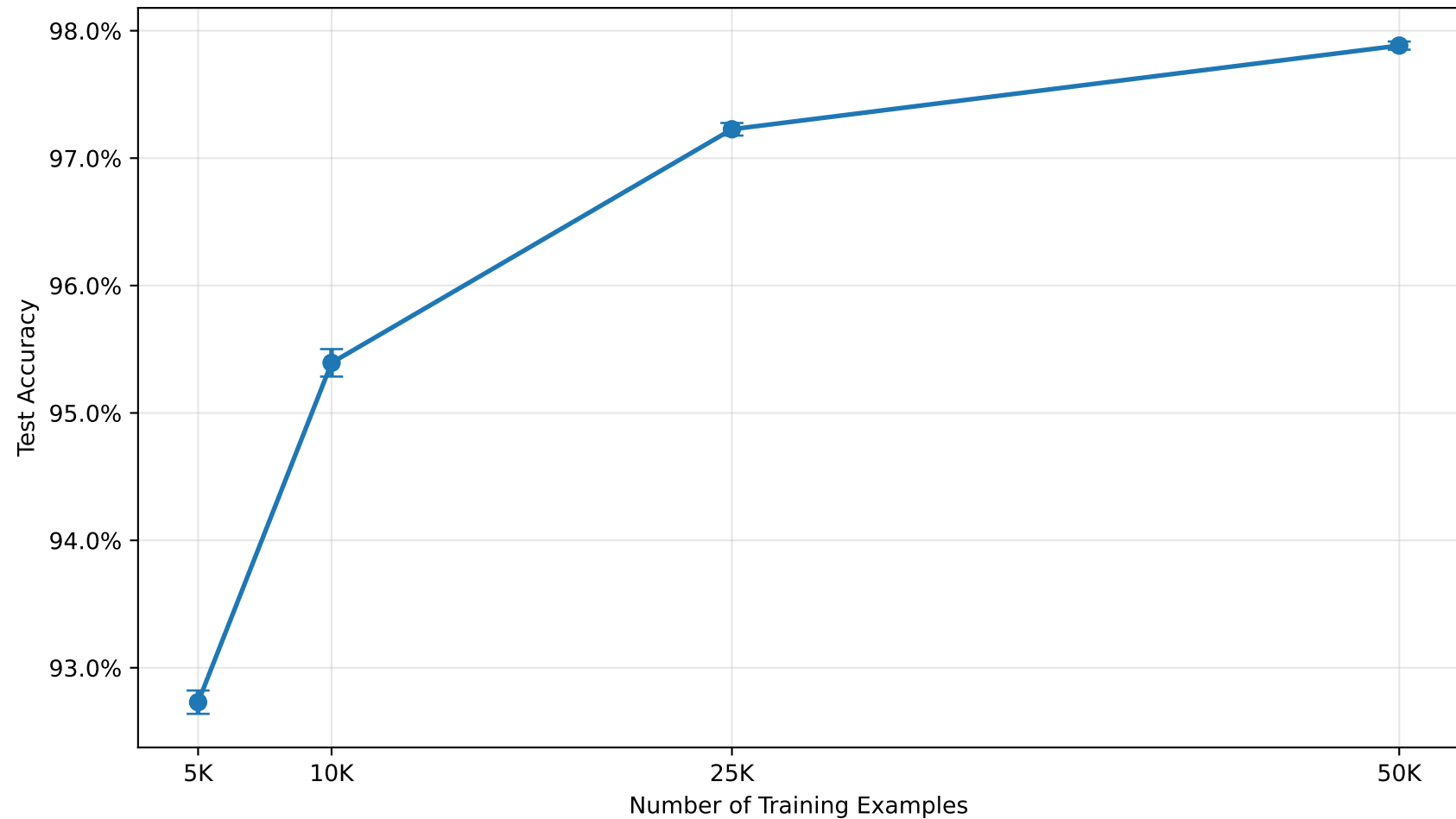
Test Accuracy by Training-Set Size
