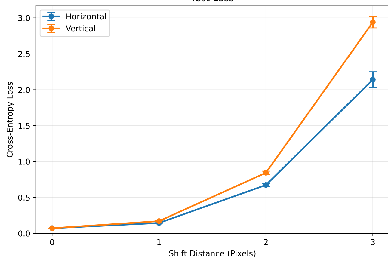
Test Loss
