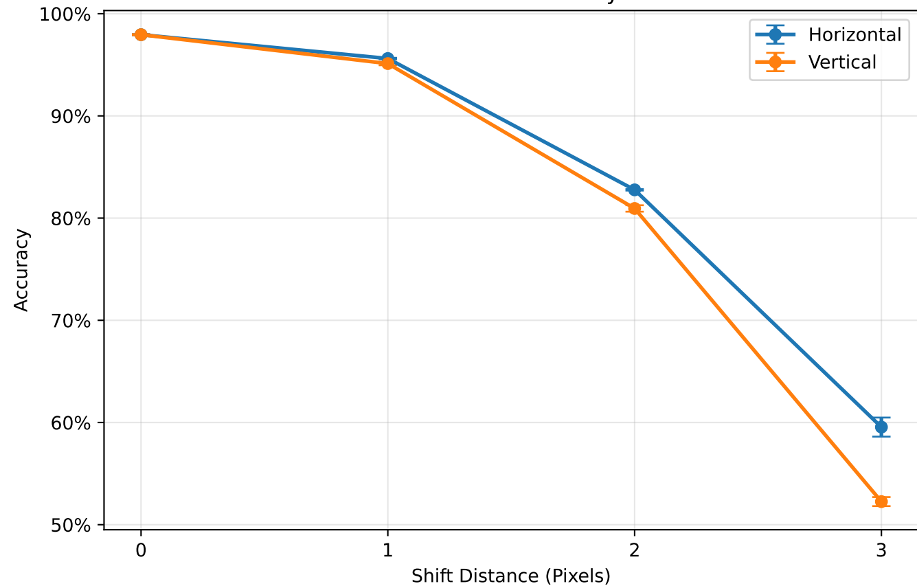
Validation Accuracy
