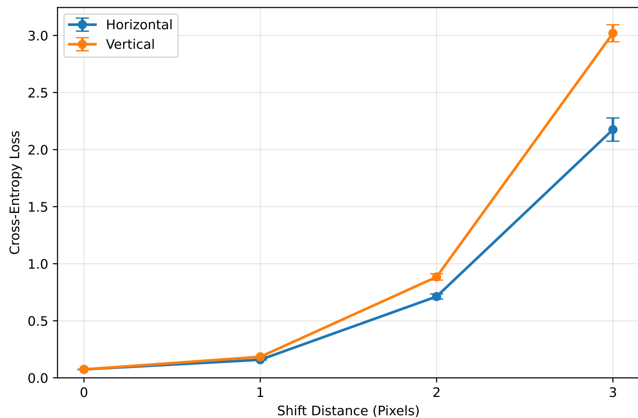
Validation Loss
