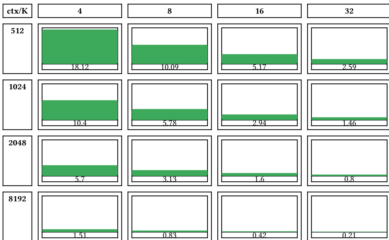
split_calls_scan (iter/s)
