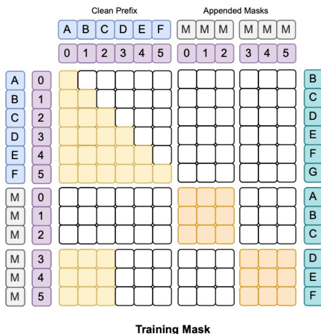
Figure 16: TiDAR training маска (diagram from TiDAR paper)
