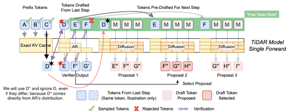
Figure 17: Anchor-TiDAR forward pass
