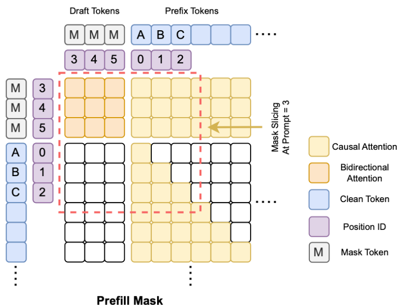
Figure 15: TiDAR prefill маска (diagram from TiDAR paper)
