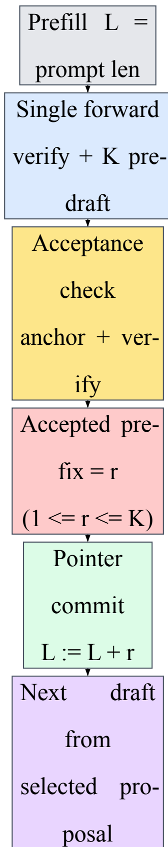
Listing 3: KV cache commit/rollback при Anchor-TiDAR: поток и pointer update
