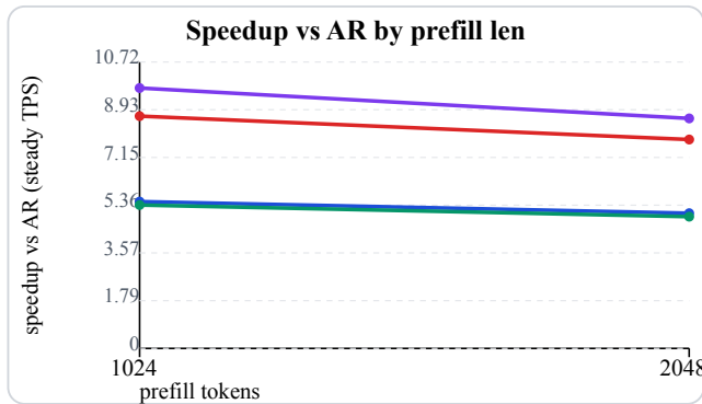
Figure 24: Head-to-head: speedup vs AR по prefill (A40 + H100)
