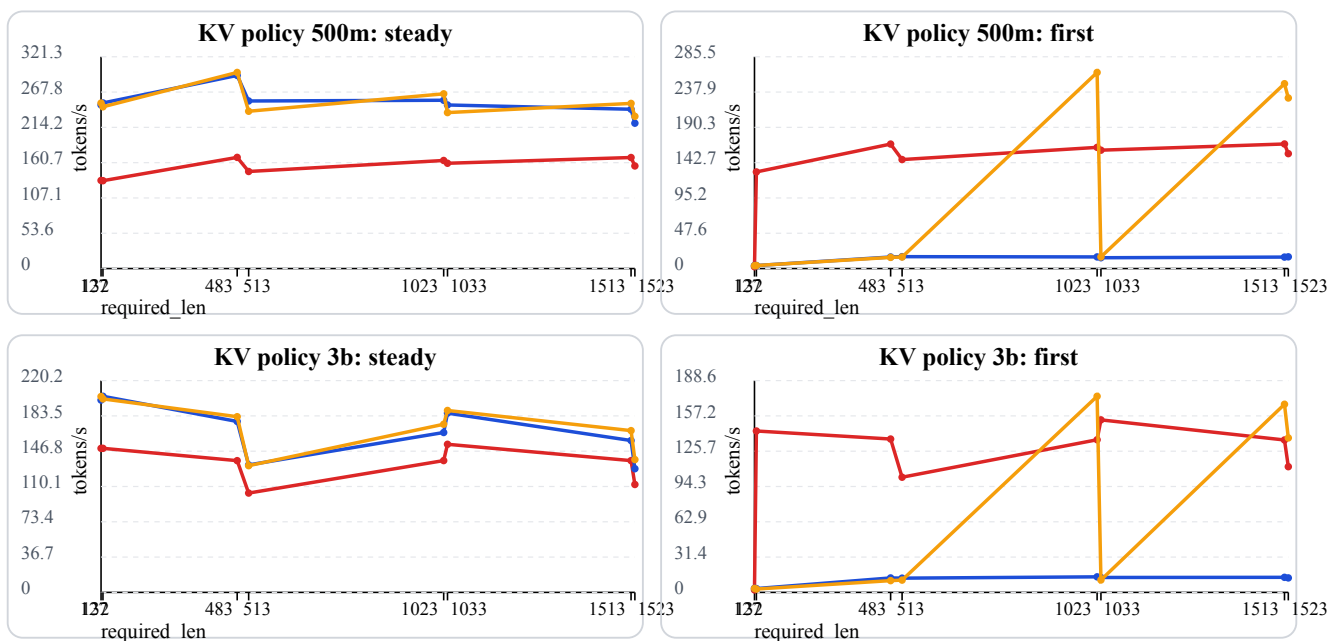
Figure 11: KV cache policy резултати (2x2) - 500m/3b, steady/first
