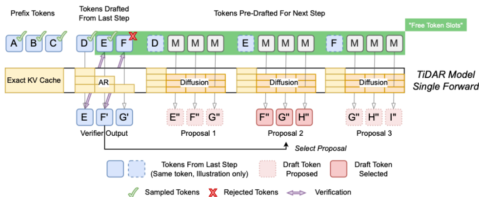
Figure 8: Single-forward layout за TiDAR verify + predraft
