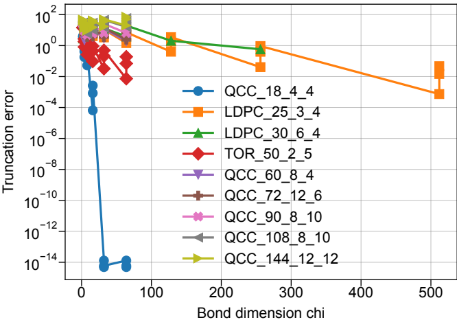
Offline truncation error vs chi
