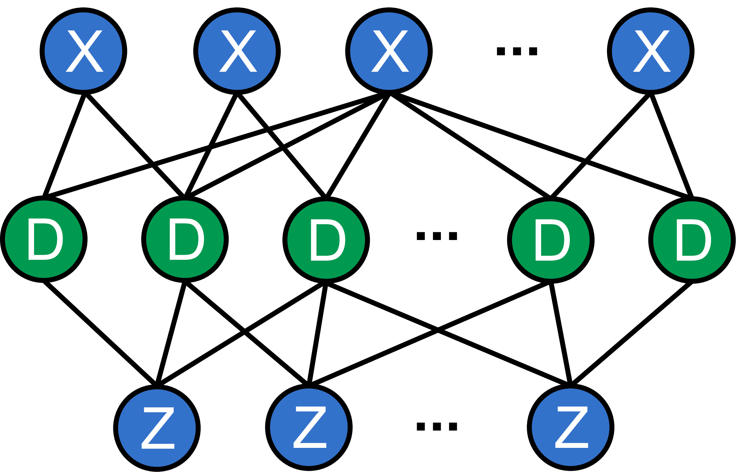
Tanner graph of general qLDPC codes
