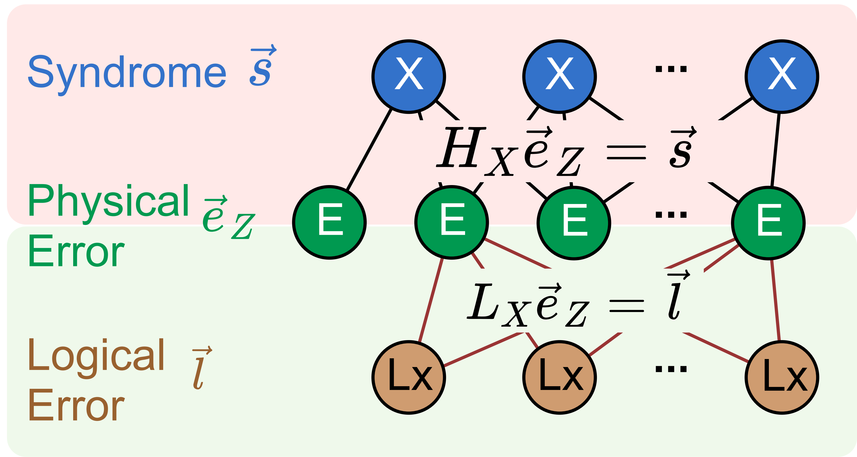
Relationship between physical errors, logical errors, and syndrome
