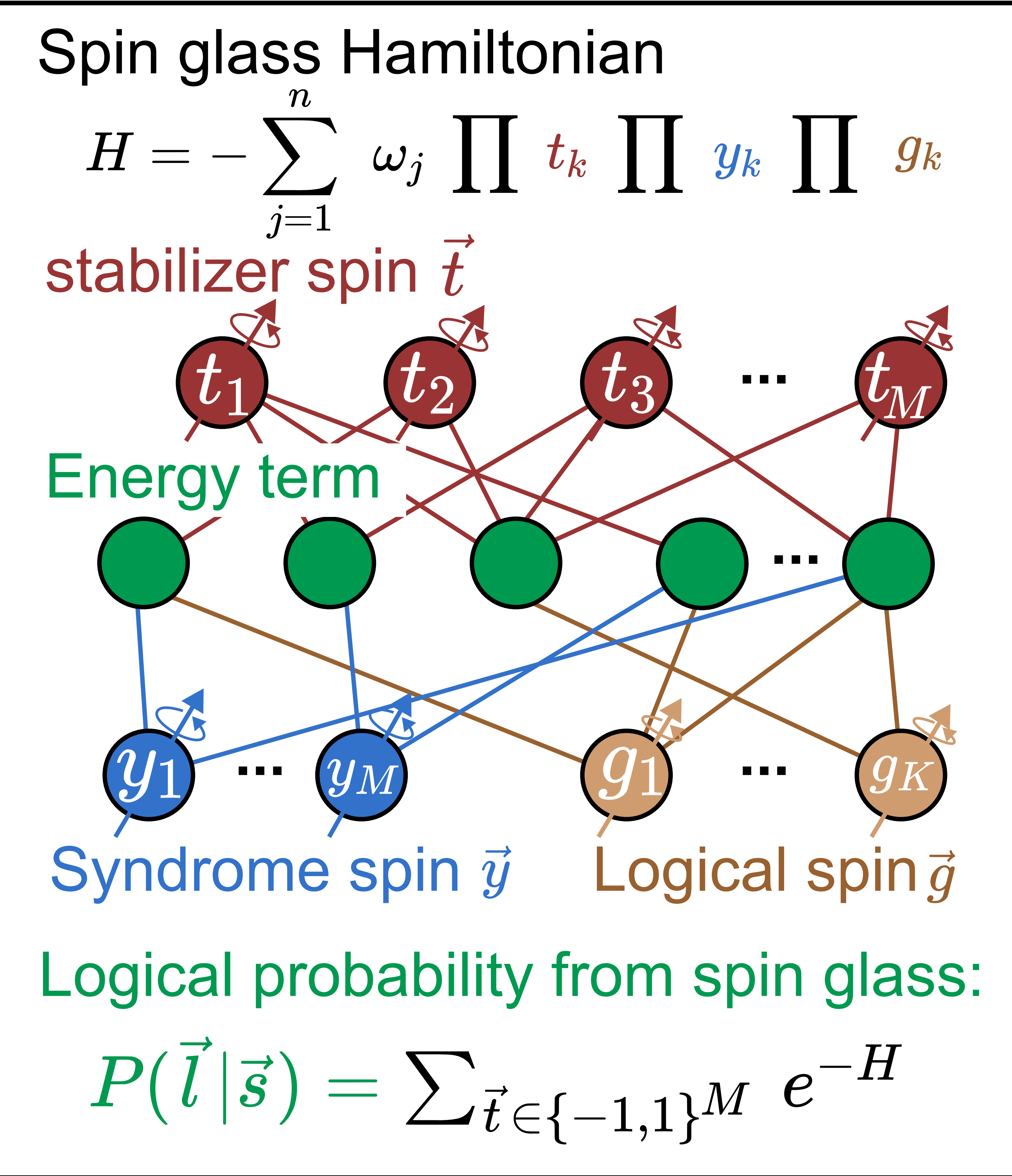
(b) Spin glass model
