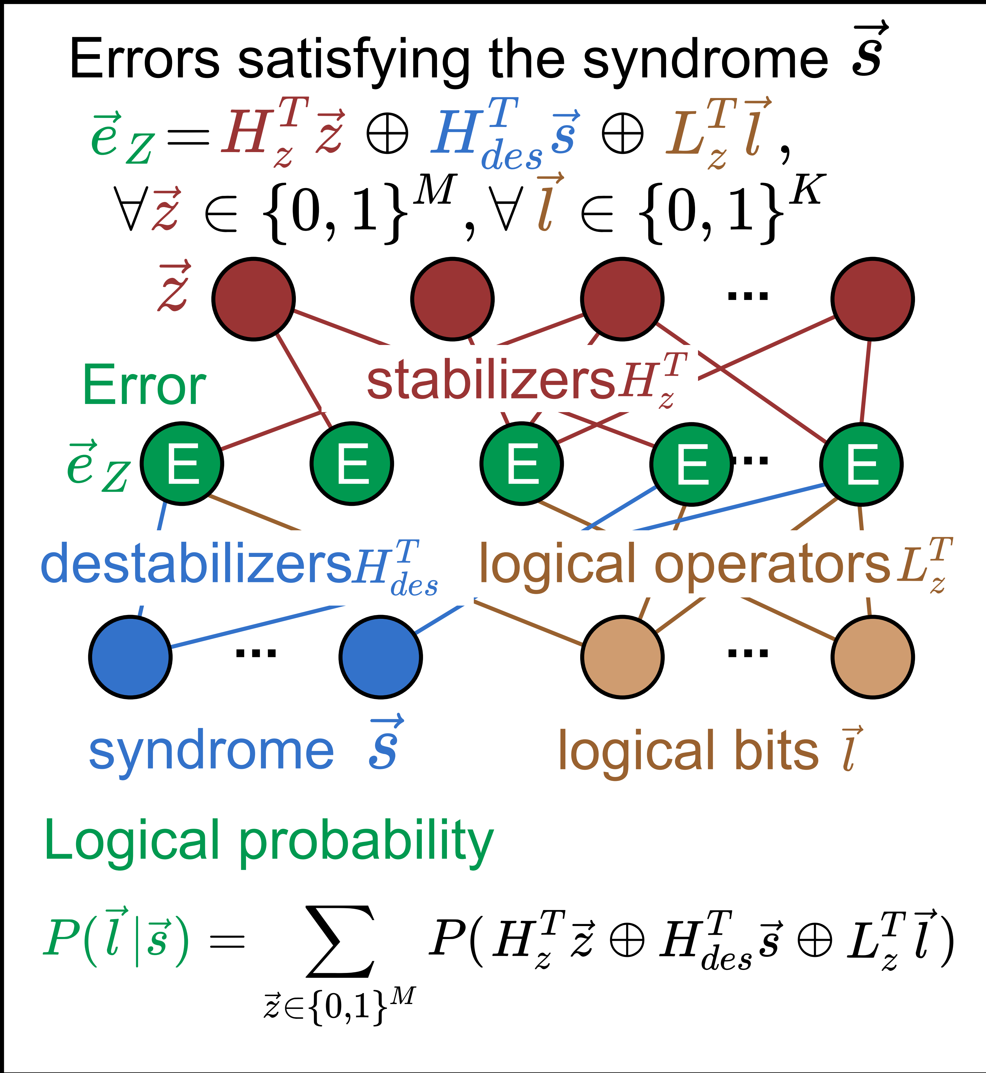
(a) qLDPC decoding
