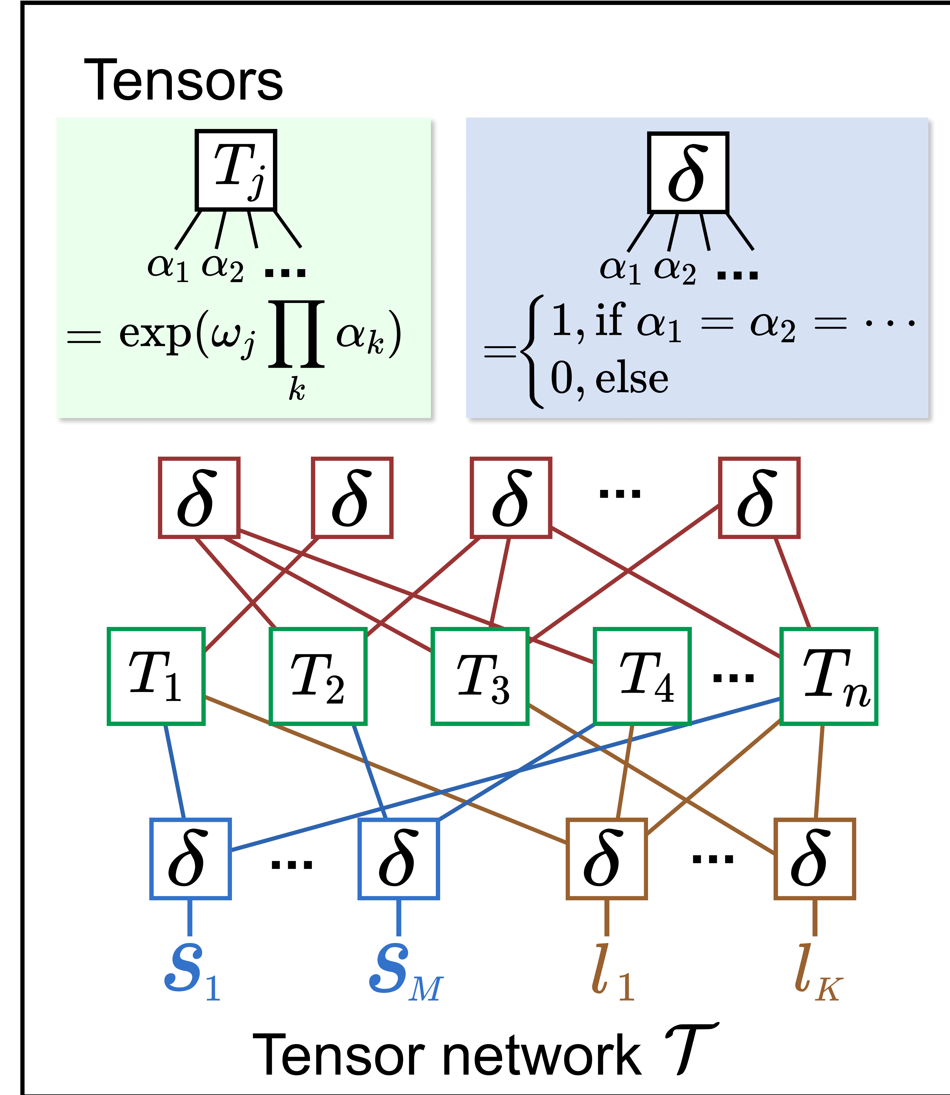
(c) Tensor network
